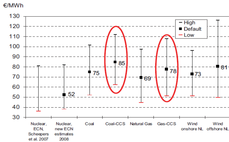
Figure 11: Integral production costs of new capacity in 2020 119
