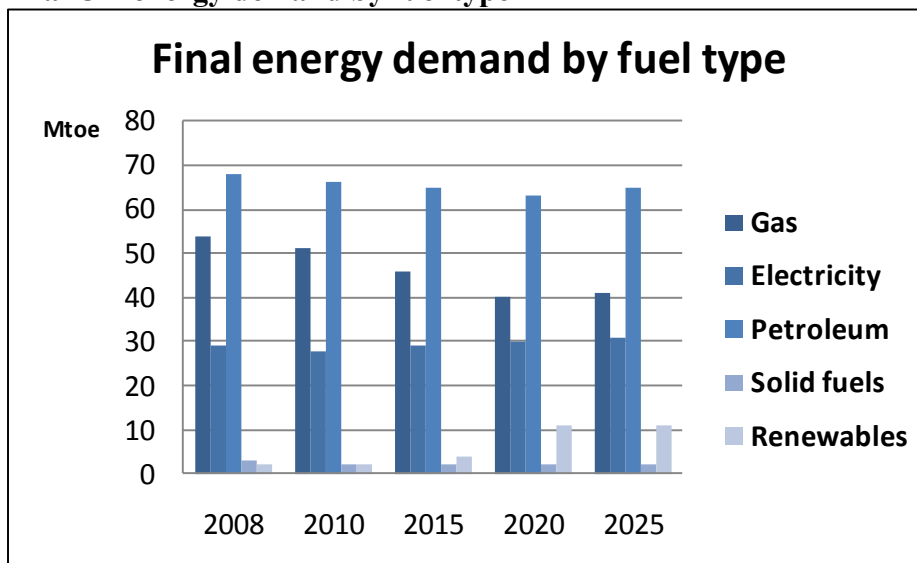
Figure 3: Final UK energy demand by fuel type
