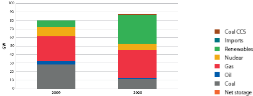
Figure 9: CCC scenario capacity mix 2020
