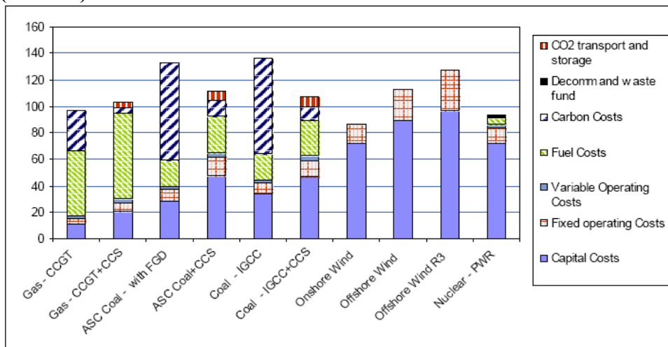
Figure 12: Levelised costs of main technologies on NOAK basis project started in 2017 (£/MWh) 120
