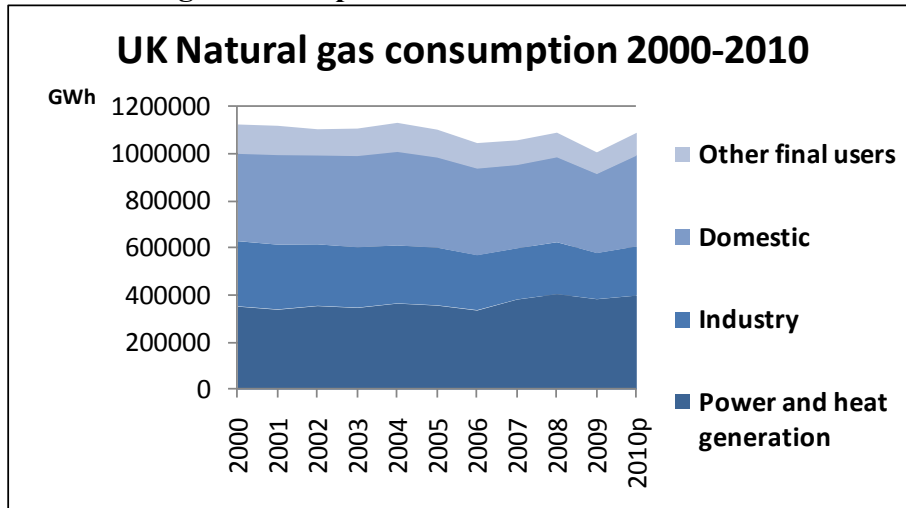
Figure 2 33 : UK natural gas consumption 2000-2010
