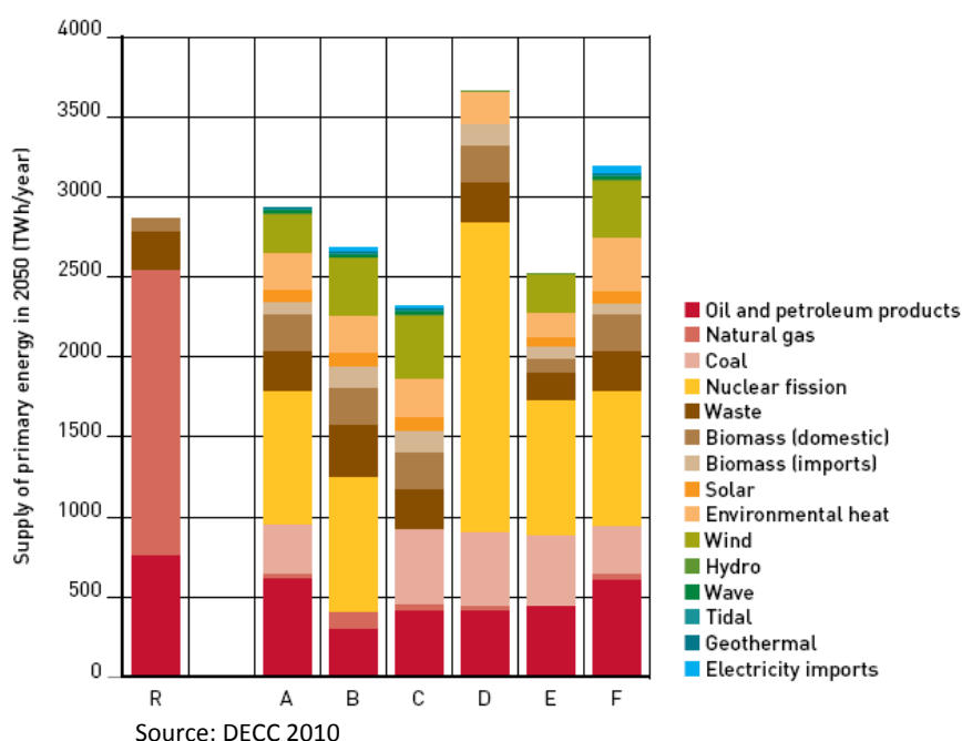
Figure 15: Summary of energy supply in 2050 across illustrative pathways
