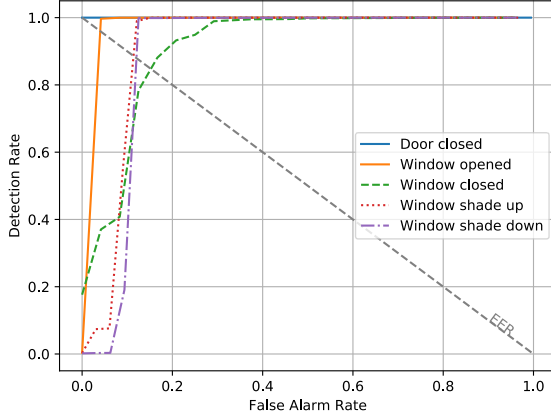
Figure 7: Receiver Operating Characteristics (ROC) curve for different events. Here we only show events with an EER significantly higher than 0 (well-classified events with an EER of 0 are a flat line at the top).
