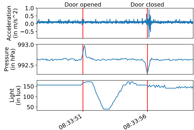
Figure 1: An example of how door events can affect different sensors. The red lines correspond to the timing of first a door opening event and then a door closing event. One can see that the door closing event has a clear effect on all three sensors, whereas the door opening event affects primarily the light and pressure sensors.
