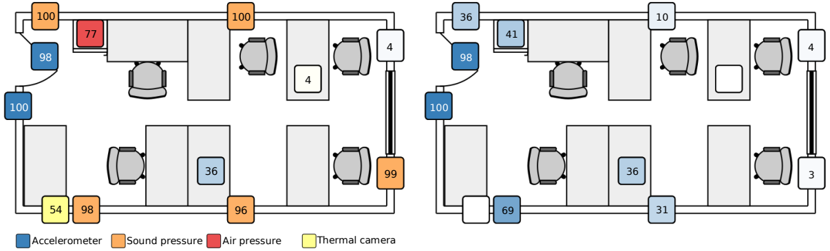
(a) Most distinctive sensor based on their position. The number given for each sensor is their maximum RMI in %. (b) Relative importance of accelerometer sensors depending on their position. Numbers are maximum RMI in %.
