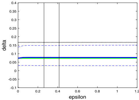
(c) n_X = 4
