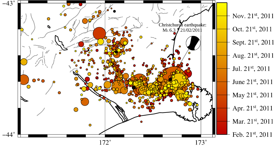
Figure 5.5: Reliably relocated earthquakes from February 21, 2011 (day of the Christchurch earthquake) to December 22 nd (day before the beginning of the swarm off-shore Christchurch city). The time of occurrence of the earthquakes are colour-coded, according to the key. The size of the symbols are scaled according to the local magnitude (see Figure 5.2 for key).
