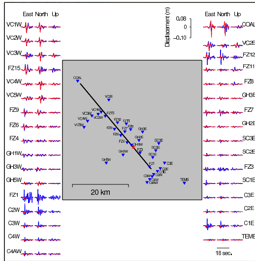
(b): Comparison of the solution seismograms from Inversion 6 with the observed data at analog stations locations. the thick black line shows the modelled fault trace. For each station, the observed seismograms are in blue and the solution seismograms are in red.
