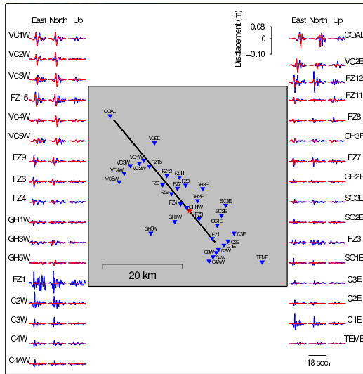
(b): Comparison of the solution seismograms from Inversion 2 with the observed data at analog stations locations. the thick black line shows the modelled fault trace. For each station, the observed seismograms are in blue and the solution seismograms are in red.
