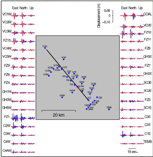
(b): Comparison of the solution seismograms from Inversion 5 with the observed data at analog stations locations. the thick black line shows the modelled fault trace. For each station, the observed seismograms are in blue and the solution seismograms are in red.
