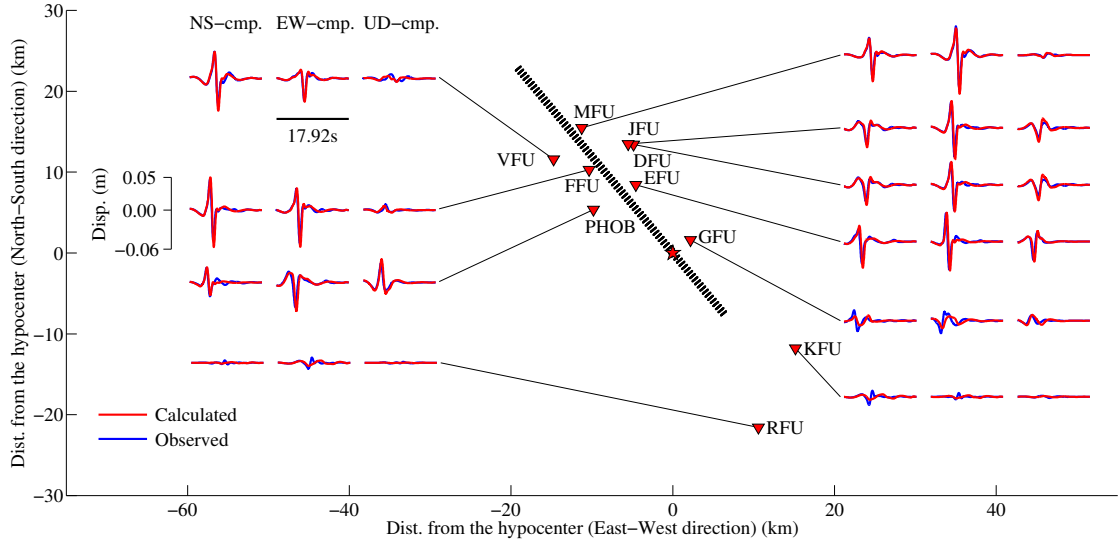
Figure A2.2: Test 2 : Comparison between the calculated displacement waveforms obtained by the inversion (ORP2) and the artificial displacement waveforms generated by the Input Rupture Process 2 (IRP2) for the 10 digital stations.
