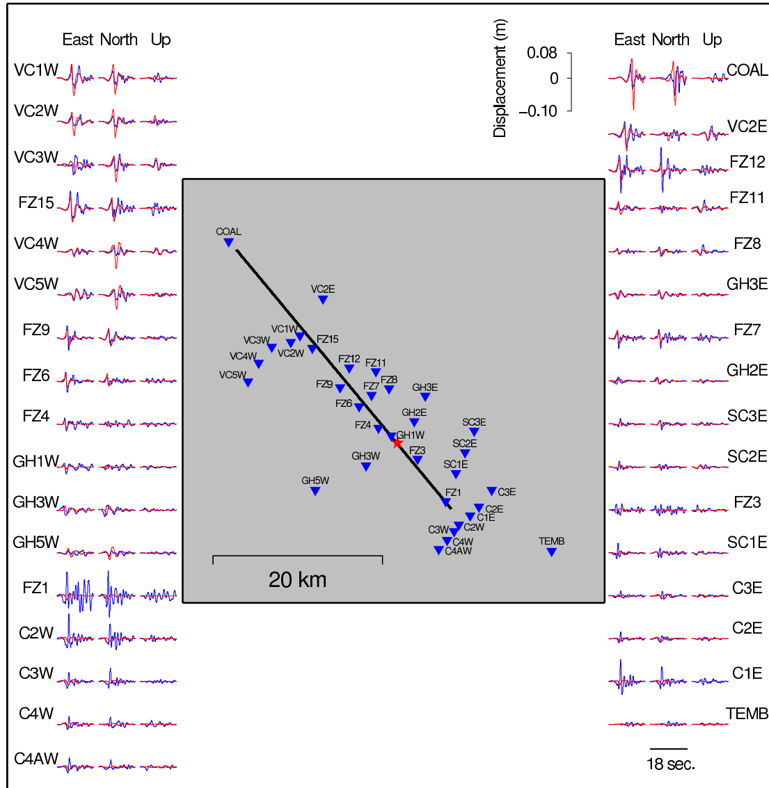
Figure 2.6: Same as Figure 5 but for the analog stations. A comparison of the observed and the solution seismograms for all inversions carried out in this study can be found in Appendix A1.
