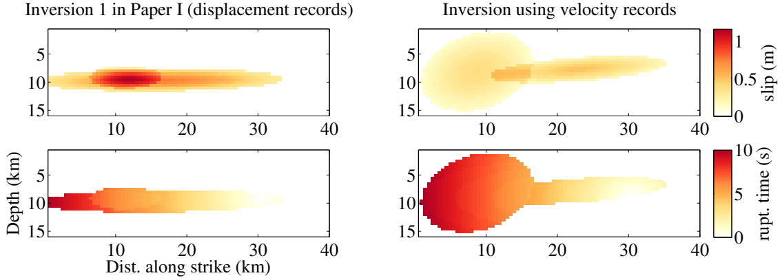
Figure 3.10: Top and bottom left figures show the final slip distribution and the isochrone for the rupture model obtained from Inversion 1 in Chapter 2, from using displacement records. Top and bottom right figures show the final slip distribution and isochrones for the rupture model obtained by inversion of velocity records.
