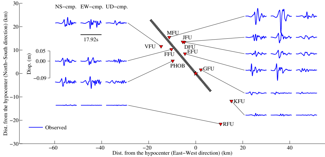
Figure 4.1: Map of the station distribution. The 3-component displacement records from the 10 digital stations of the GEOS network used to perform the dynamic inversion are shown by the blue trace. The red star shows the location of the epicentre and the black dashes show a surface projection of the fault plane.
