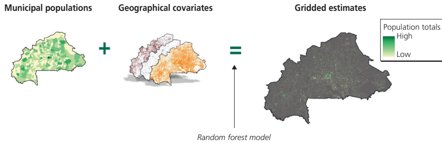
Figure 3. Top-down modelling of the disaggregation of national population totals at the grid-cell level
