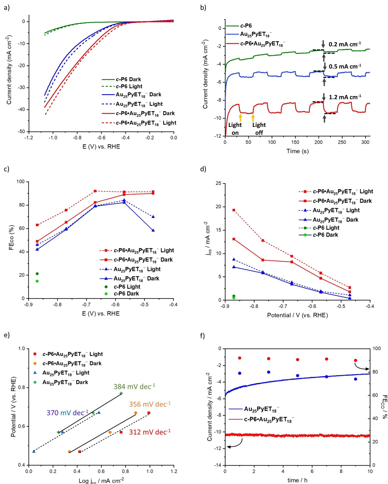
Figure 6. Electrocatalytic and photo-coupled electrocatalytic CO 2 reduction performances. a) LSV curves, b) Photocurrent response at -0.67 V vs. RHE, c) FE CO and d) j CO of c-P6, Au 25 PyET 18 - and c-P6•Au 25 PyET 18 - under dark and light conditions. e) Tafel plot under dark and light conditions and f) Stability test at -0.67 V vs. RHE under light illumination for Au 25 PyET 18 - and c-P6•Au 25 PyET 18 - .
