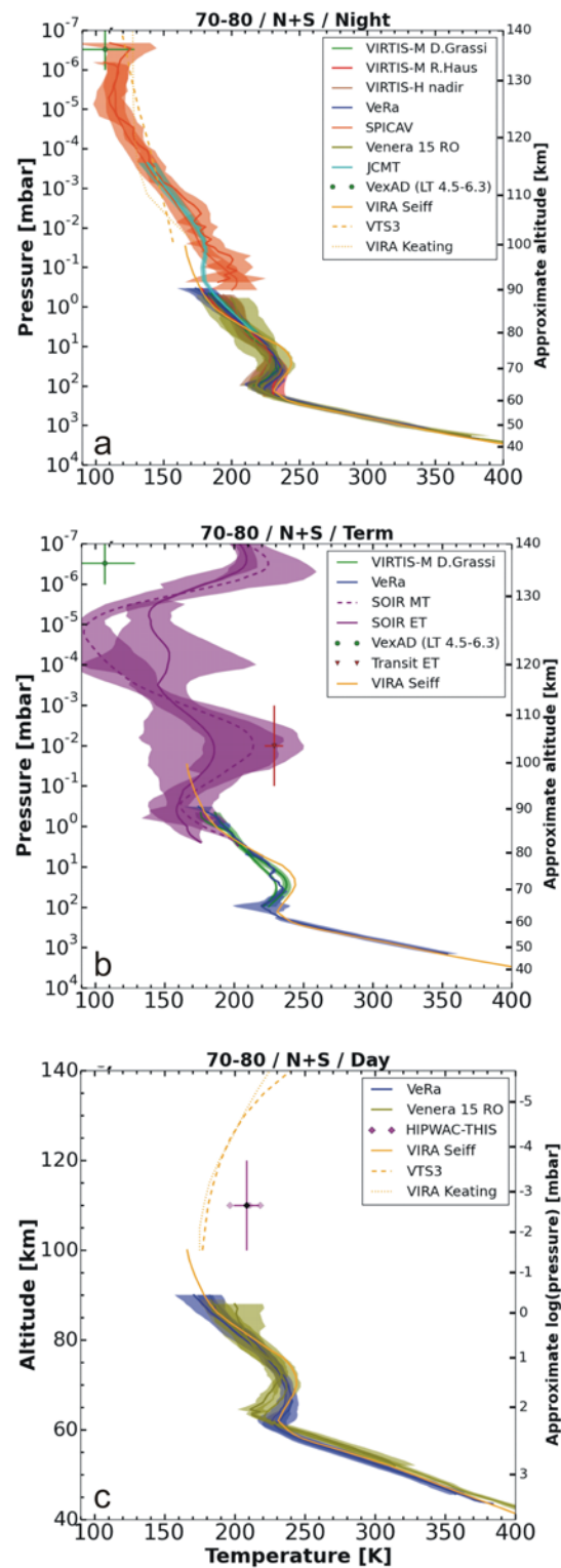
Figure 18: same as Figure 15 but for combined temperature profiles from the Northern and Southern hemispheres between the 70° and 80° latitude. Panel (a): night side, panel (b): terminators, panel (c) day side.
