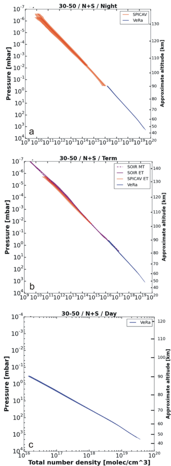
Figure 21: same as Figure 20 but for the latitude bin 30° to 50°. Panel (a): night side, panel (b): terminator zones, panel (c): day side. The colored areas mark the one standard deviation uncertainty of the average profiles for each experiment. Approximate altitudes are shown on the right hand vertical axis.
