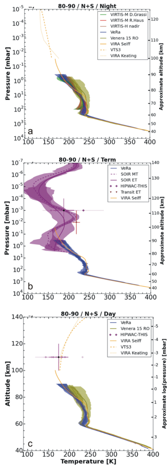
Figure 19: same as Figure 15 but for combined temperature profiles from the Northern and Southern hemispheres between 80° and 90° latitude. Panel (a): night side, panel (b): terminators, panel (c) day side.
