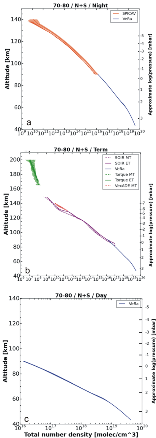
119 120 Figure 28: same as Figure 26 but for the high latitudes (70° to 80°). Panel (a): night side, panel (b) 121 terminator zone, panel (c) day side.
