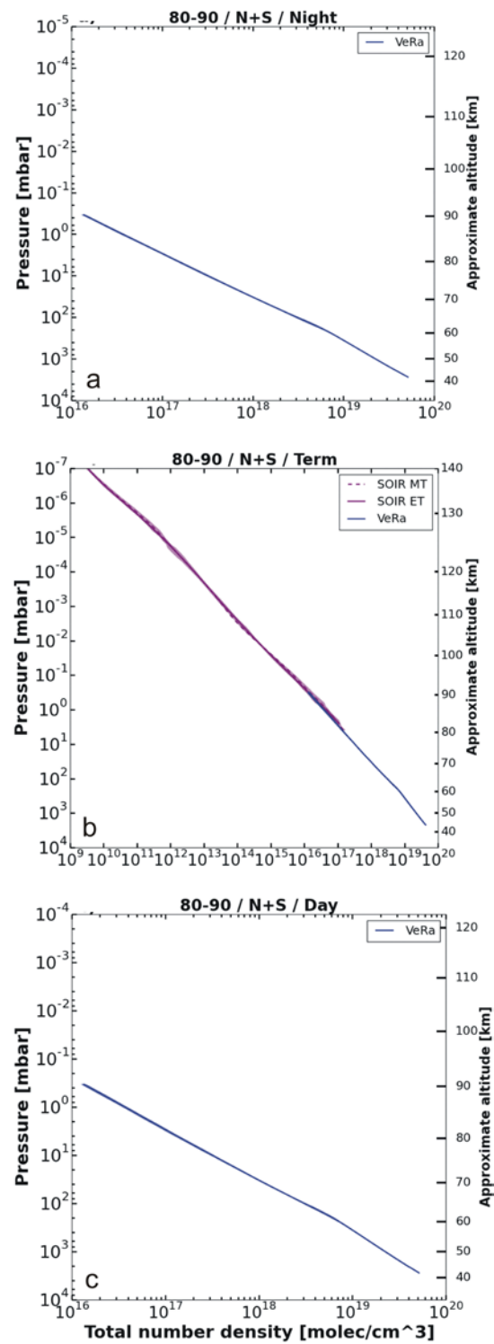
Figure 24: same as Figure 21 but for the latitude bin 80° to 90°. Panel (a): night side, panel (b): terminator zones, panel (c): day side. The colored areas mark the one standard deviation uncertainty of the average profiles for each experiment. Approximate altitudes are shown on the right hand vertical axis.
