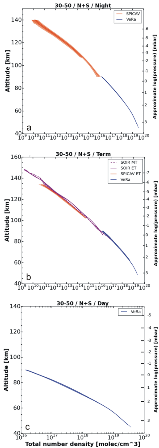
Figure 26: same as Figure 25 but for the mid-latitudes (30° to 50°). Panel (a): night side, panel (b) terminator zone, panel (c) day side.
