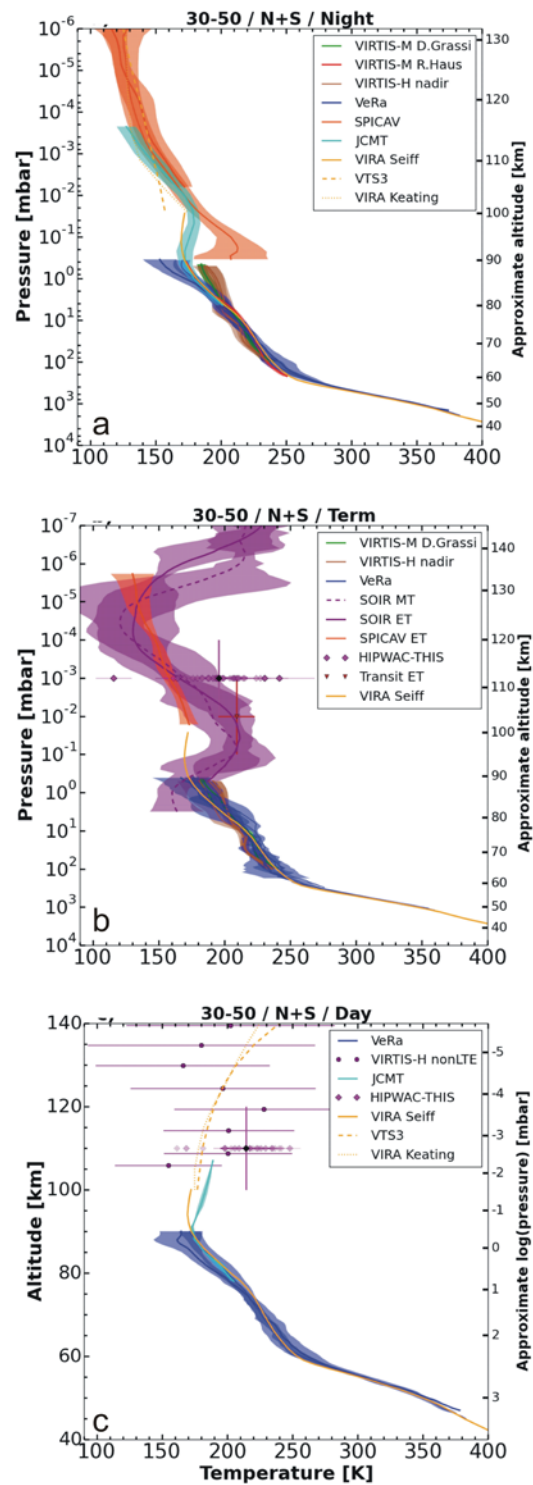
Figure 16: same as Figure 15 but for combined temperature profiles from the Northern and Southern hemispheres between 30° and 50° latitude. Panel (a): night side, panel (b): terminators, panel (c) day side.
