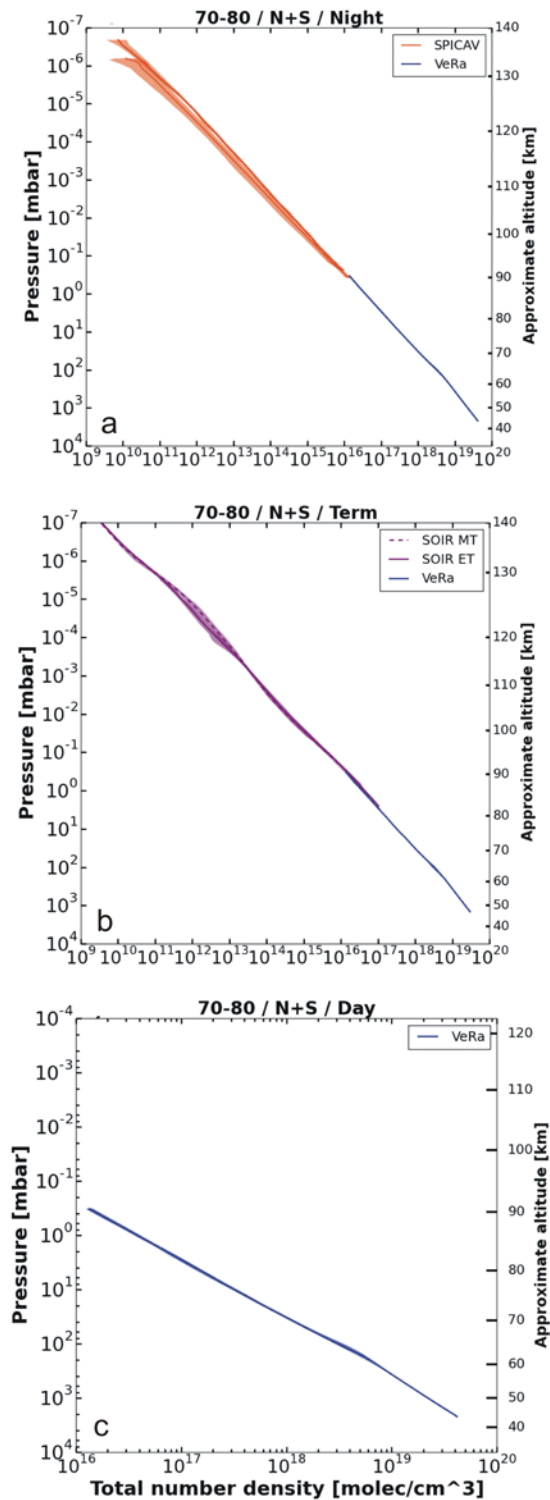
100 Figure 23: same as Figure 21 but for the latitude bin 70° to 80°. Panel (a): night side, panel (b): terminator 101 zones, panel (c): day side. The colored areas mark the one standard deviation uncertainty of the average 102 profiles for each experiment. Approximate altitudes are shown on the right hand vertical axis.
