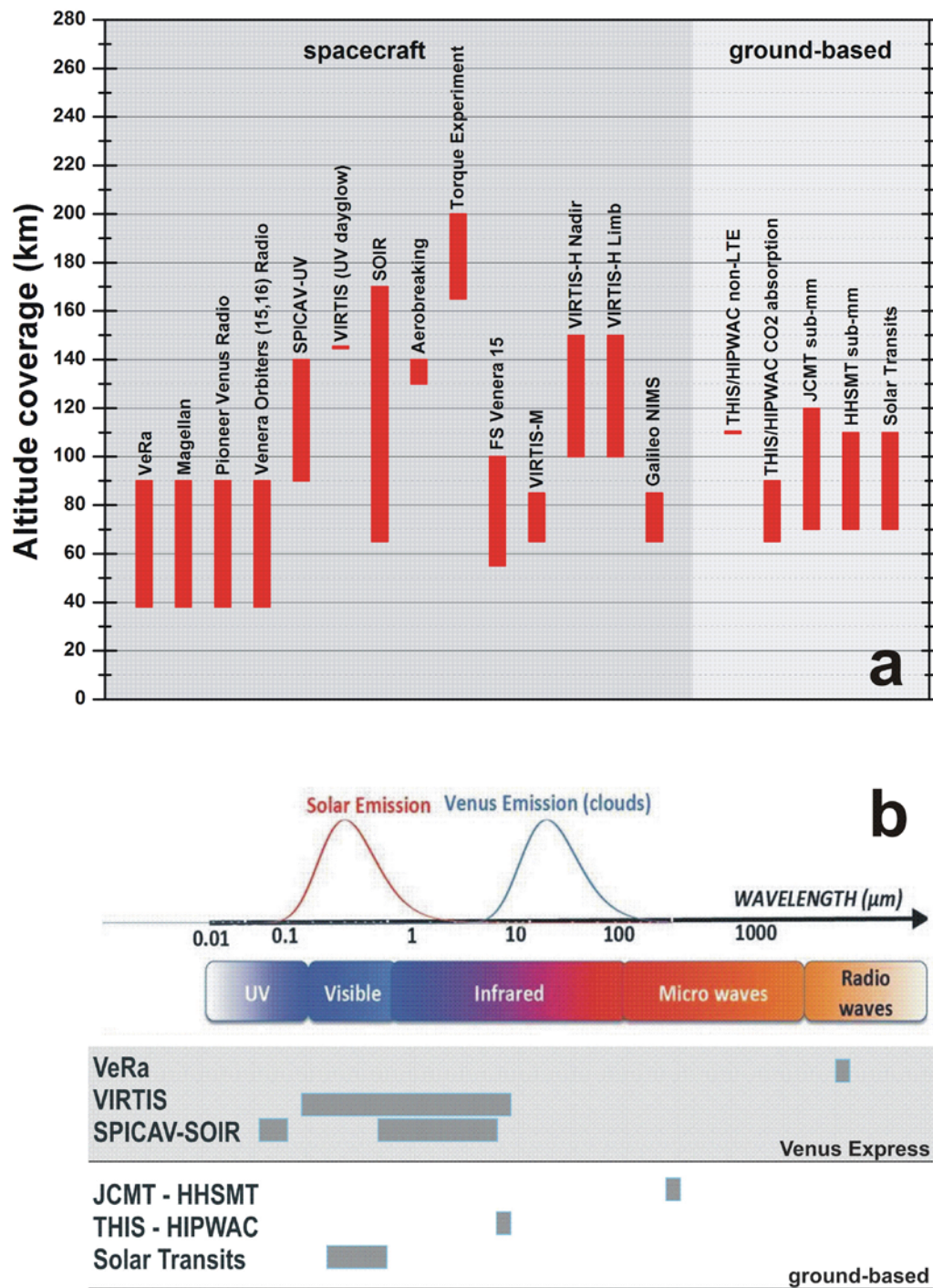
Figure 1: Panel (a): vertical coverage of the post-VIRA atmospheric structure experiments. Panel (b): spectral ranges of the experiments considered in this study
