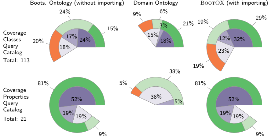
Figure 13: Coverage of terms from the Statoil query catalog with terms from ontologies. Inner pie charts show coverage by lexical confidence using I-SUB [80]: ■ in [0.9, 1.0] , ■ in [0.8, 0.9] , □ in [0.6, 0.8] . Outer pie charts represent the manual verification of the quality of the terms with a coverage above 0.6: ■ true positive , ■ semi-true positive , ■ false positive . Note that semi-true positives are not clear-cut cases where the ontology term has a broader or narrower meaning with respect to the query term.
