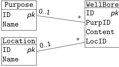
(a) Database Schema
