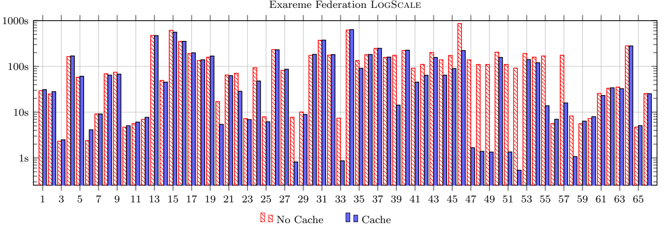
Figure 17: Execution Times for Federated Scenario (With and Without Query Cache)
