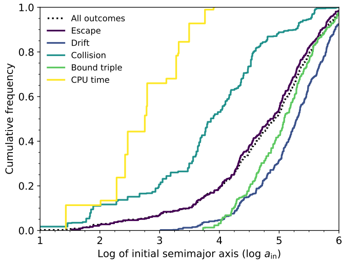
Fig. 10. Origin of destabilised triples and their outcomes. Where as drifters and long-lived triples originate from triples with large initial orbital separations, colliding stars and CPU-limited systems come from compact initial triples.
