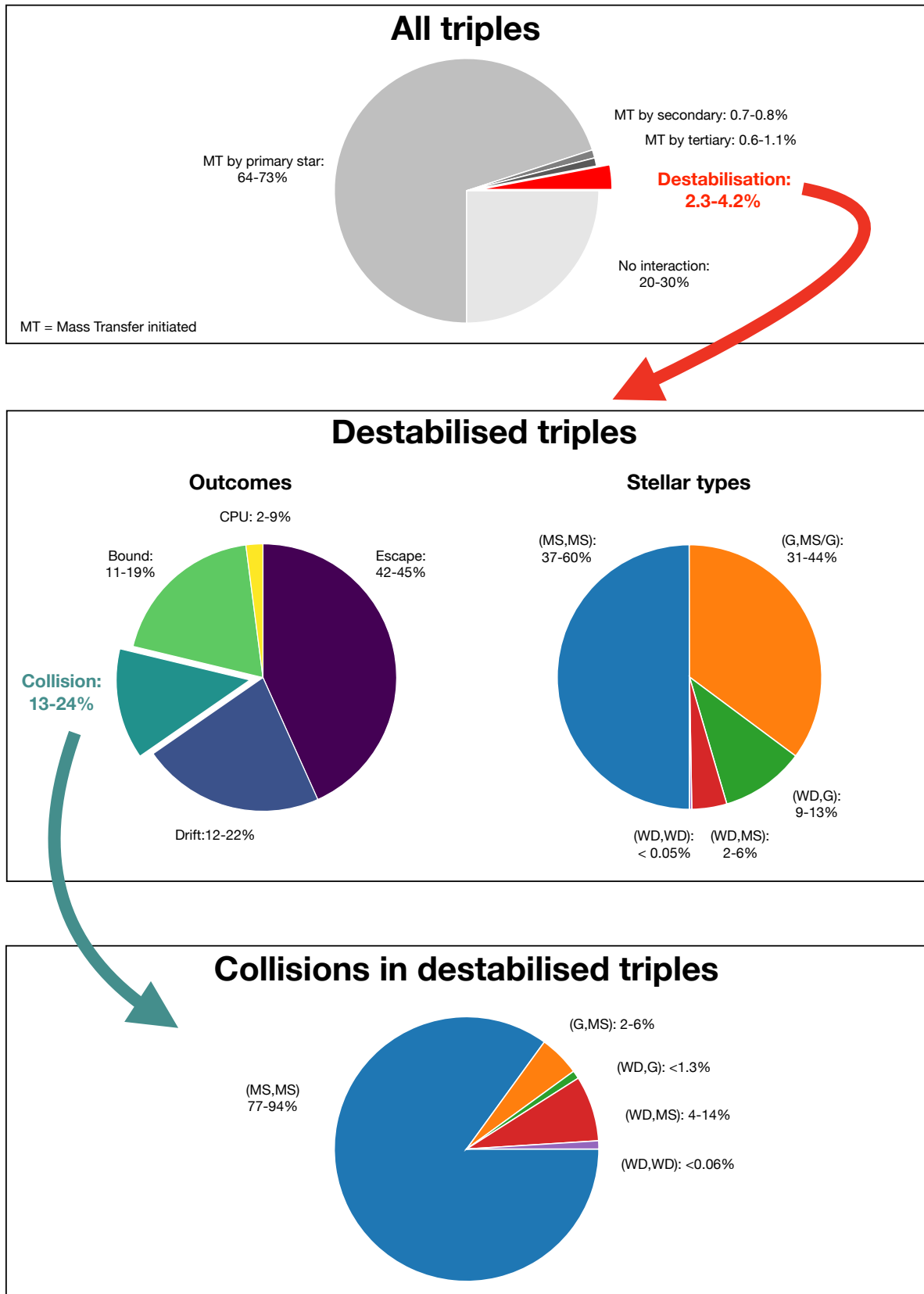
Fig. 1. Overview of the outcome of triple evolution. About 2–4% of triples destabilise by themselves during their evolution ( top panel ). These triples commonly consist of three MS stars or contain one or two giant stars ( middle right panel ). The outcome of the destabilised phase is often an ejection of one of the stars, but collisions are common as well ( middle left panel ). Collisions preferably occur between MS stars ( bottom panel ). Fractions are based on our most advanced N -body simulations that includes stellar evolution.
