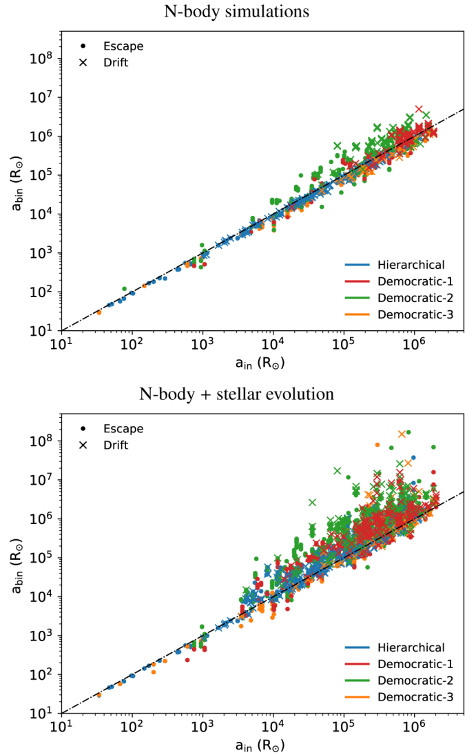
Fig. 8. Change in orbital separation for destabilised triples that unfold into a binary and single star. The x -axis shows the orbital separation of the inner orbit at the onset of the instability, and the y -axis shows the post-interaction orbital separation of the binary. The results of the pure N -body simulations are shown in the top panel , those of simulations that include stellar evolution are shown on the bottom . The black dashed line represents no change in the orbital separation. The figure shows that besides adiabatic wind mass losses leading to orbital widening, ejecting a star from the inner orbit also tends to lead to orbital widening (see text). The two panels represent model OBin. Model T14 and E09 show qualitatively similar trends.
