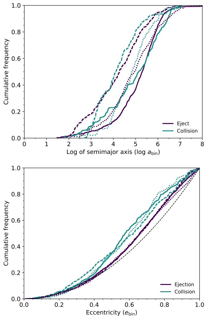
Fig. 14. Properties of the (isolated) binaries that are formed from destabilised triples. Solid, dashed, and dotted line styles represent the N -body + SE models for the initial population of triples OBin, T14 and E09, respectively. The black dashed line represents a thermal distribution of eccentricities.
