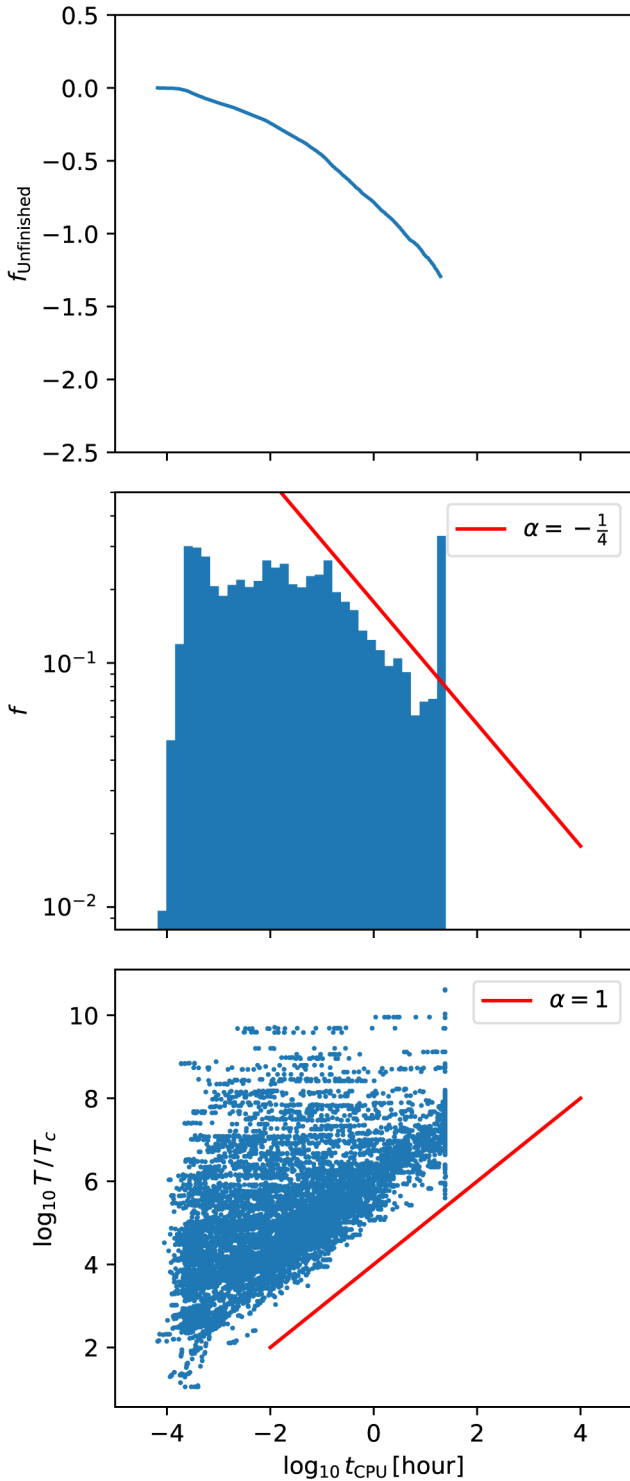
Fig. D.1. For the ensemble of triples which included full stellar evolution, we plot 1) the fraction of unfinished simulations vs. CPU time (top), 2) histogram of CPU times (middle), and 3) simulated physical time normalised by the crossing time vs. CPU time (bottom). The red lines represent estimates of the slopes in the data, with coefficient \alpha .
