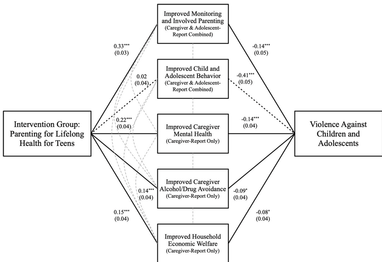
Fig. 1. Structural Equation Model of Program Mediators, Notes: *** p < 0.001 , ** p < 0.01 , * p < 0.05 . All coefficients shown are standardized.
