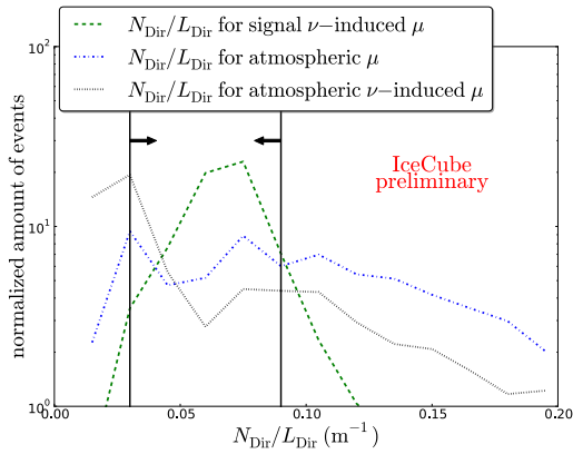
Figure 6: The normalized distributions for N_{\text{Dir}}/L_{\text{Dir}} . The vertical lines show the cut values used in this analysis and the arrows indicate the parameter region that is retained.
