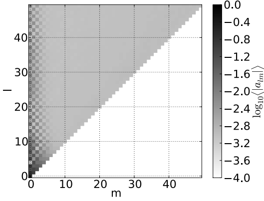
Figure 3: Shown is the logarithm of the absolute value for all coefficients in the \ell - m -plane. The absolute value was averaged over 1000 pure signal skymaps.
