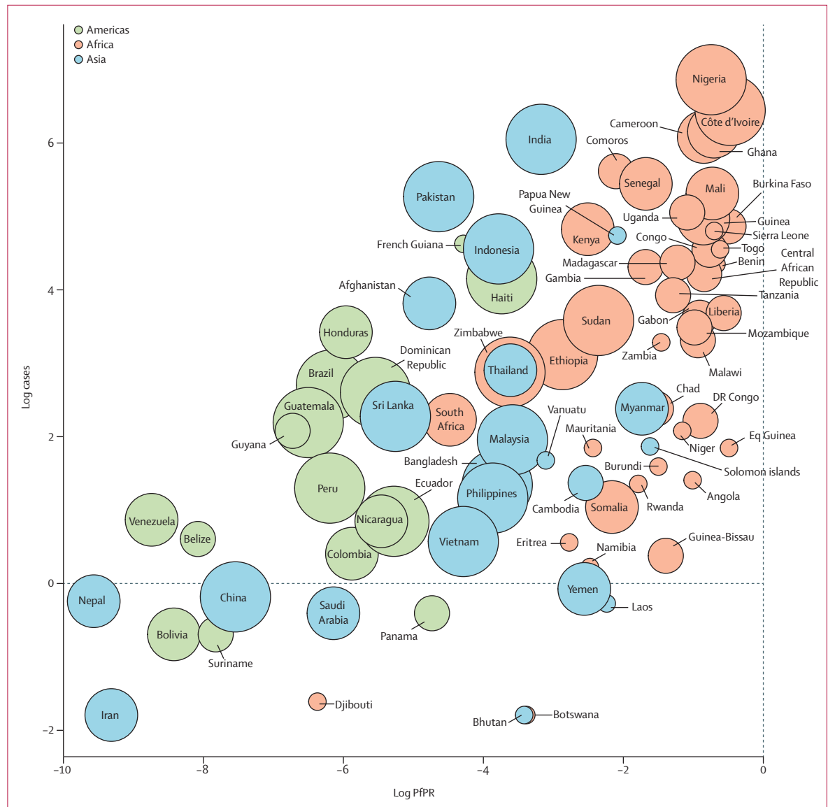
Figure 3: Plasmodium falciparum prevalence in 2010 versus average annual number of P. falciparum cases imported to non-endemic countries for all endemic countries, 2005–15
