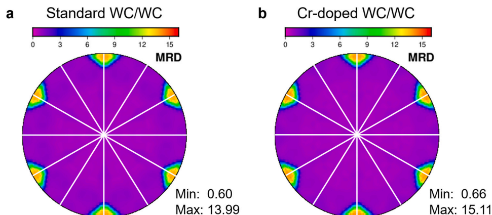
Fig. 3. 90^\circ axis-angle distributions for the standard WC/WC and Cr doped WC/WC boundaries, with minimum and maximum MRD values indicated.
