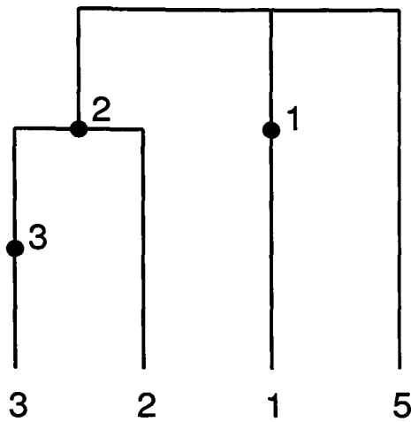
Figure 5.2: A simple gene tree, mutation 2 is the selected mutation.
