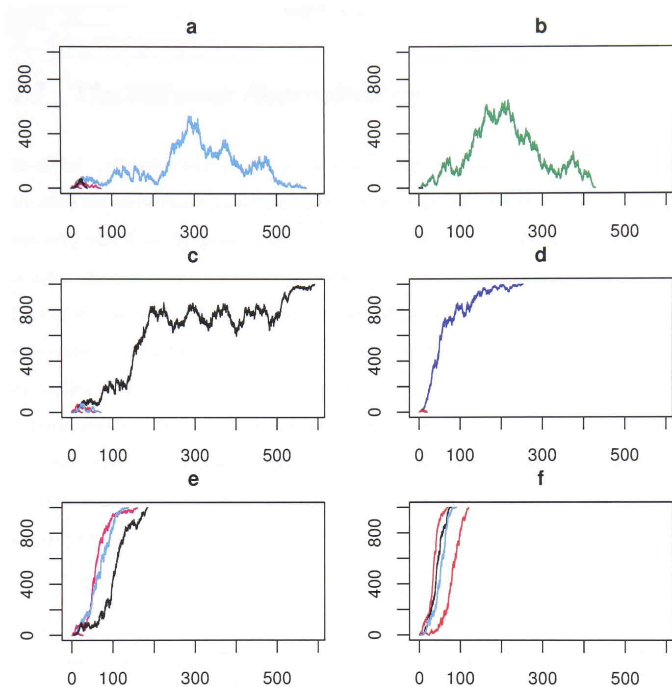
Figure 2.2: A sample of twenty trajectories generated by a forward in time Moran model ( N = 1000 ) from an initial occurrence of the mutation in one individual for a variety of genic selection coefficients a) neutral s_N = 0 , b) s_N = 0.0001 , c) s_N = 0.001 d) s_N = 0.025 e) s_N = 0.05 , f) s_N = 0.1 . Time is given along the x -axis and number of the selected mutation in the population on the y axis
