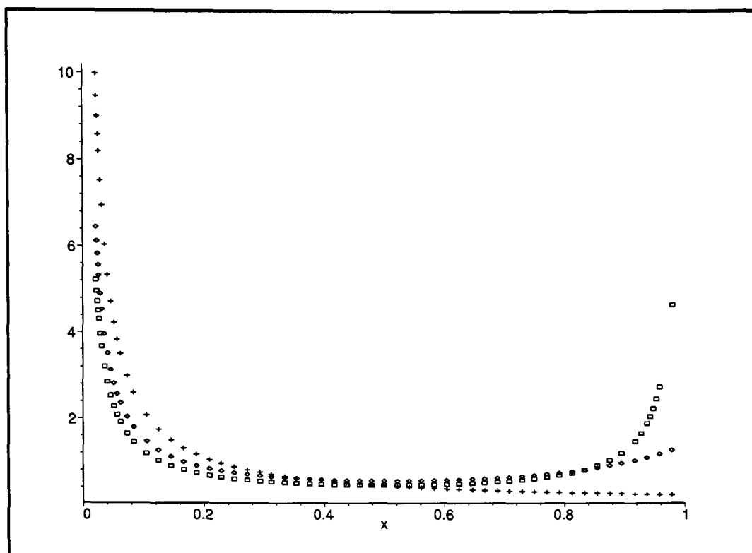
Figure 3.1: The population frequency spectrum of a derived mutation under a variety of genic selection coefficients \beta = 0 (+), \beta = 10 ◇, \beta = 100 □
