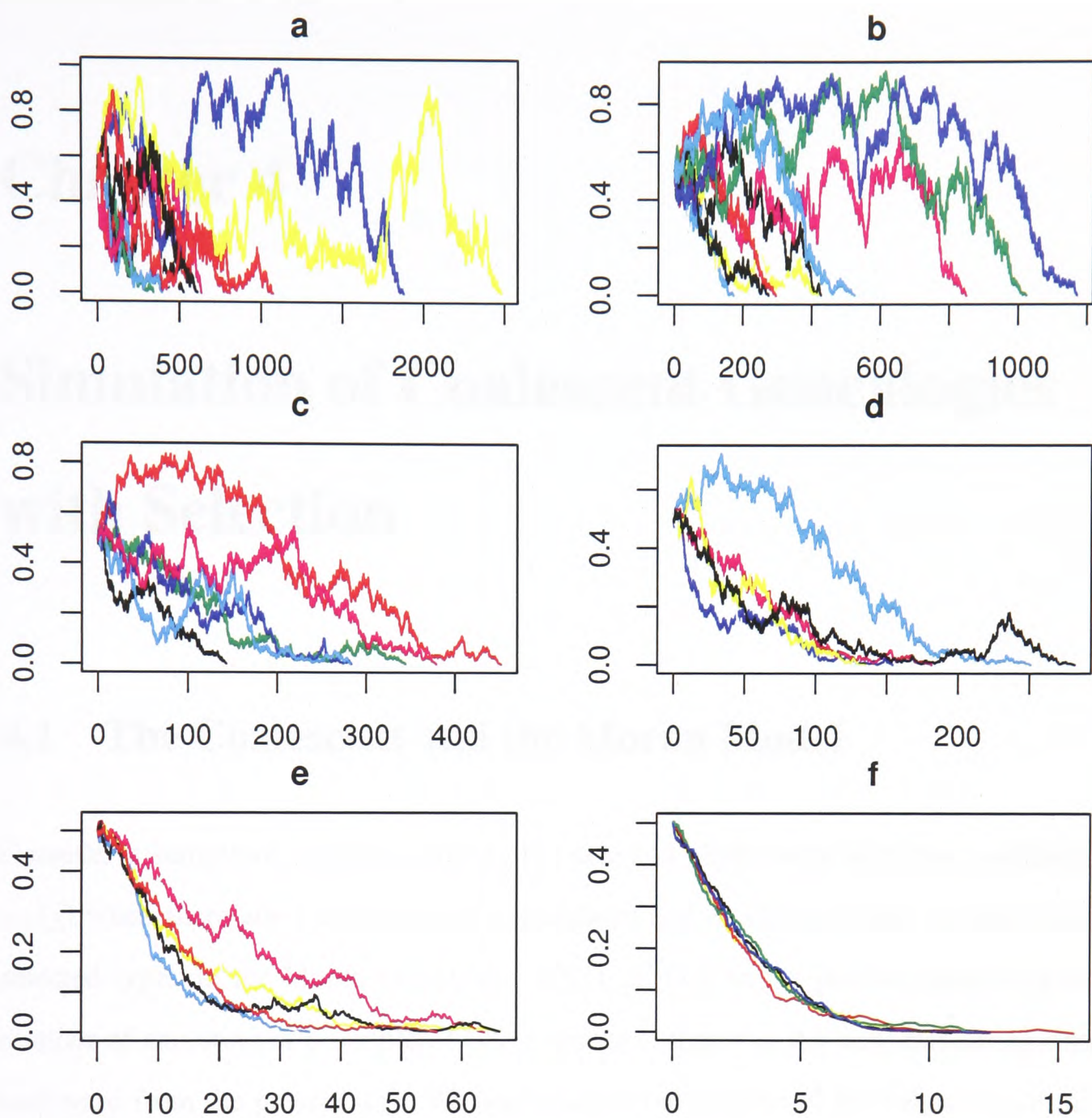
Figure 3.7: A sample of twenty trajectories generated by a backward in time Moran model conditioned on loss from a present day frequency of .5 in a population of 1000 for a variety of selection coefficients a) neutral \beta = 0 , b) \beta = 0.1 , c) \beta = 1 d) \beta = 25 e) \beta = 50 , f) \beta = 100 . Time is given along the x-axis and number with the selected mutation in the population on the y-axis
