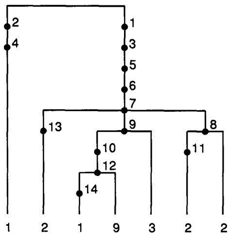
Figure 2.4: The gene tree for the example data set. The black dots are the mutations with their reference number written beside them, and the multiplicities of the various types are given at the bottom.
