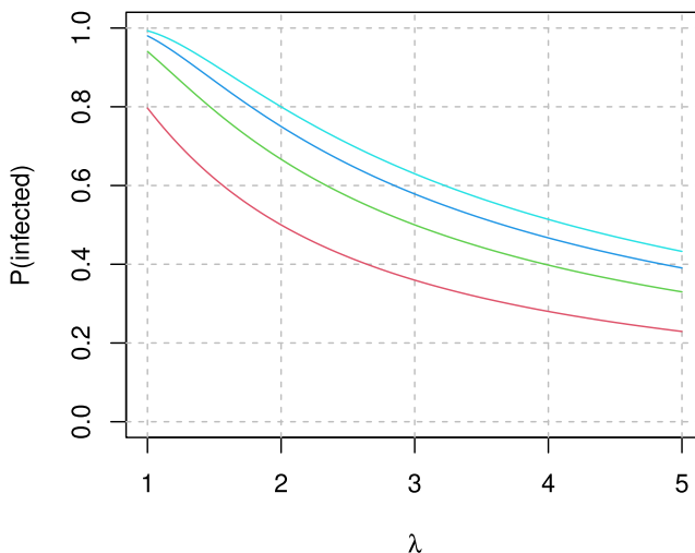
Figure 8. Final proportion infected against \lambda for R_0 = 2, 3, 4, 5 (ascending, red, green, blue, and turquoise), for Susceptible Exposed Infectious Recovered (SEIR) epidemic models with susceptibility or mixing rates varying across individuals. The age band dependent variability used by Scientific Advisory Group for Emergencies (SAGE) models in the UK corresponds to \lambda \approx 1.2 . Realistic estimates seem to be in the range 2.5–5.
