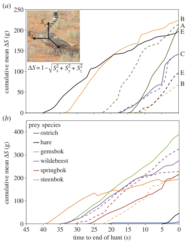
Figure 2. Mean cumulative VeSBA ( \Delta S , g) of successful (solid lines) and unsuccessful (dashed lines) cheetah hunts against time ( n = 35, 30 Hz) for (a) steenbok hunts for cheetah individuals A–E and (b) different prey species chased. Mean r^2 of linear regressions was 97.4 \pm 2.75\% , S_x , S_y and S_z are orthogonal components of static acceleration.
