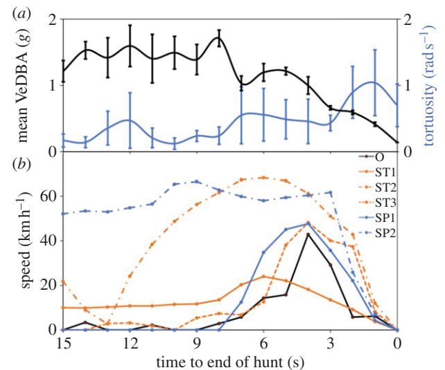
Figure 1. (a) Mean VeDBA ( g , 9.81 \text{ m s}^{-2} ) and angular velocity ( \text{rad s}^{-1} ) against time ( n = 35 , 30 Hz) during the last 15 s of cheetah chases. Error bars represent standard errors; (b) Speed ( \text{km h}^{-1} ) against time (s) ( n = 6 , 1.0 Hz) across the last 15 s of cheetah chases for ostrich (O), steenbok (ST1, ST2 and ST3) and springbok (SP1 and SP2). Hunts O, ST2 and ST3 were successful.
