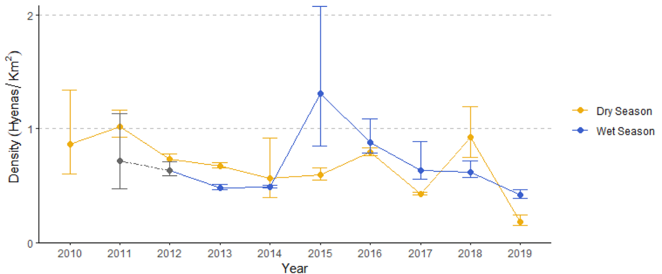
FIGURE 3 | Density estimates ( \hat{D} ) per season and per year for 2010–2019 including 95% credible intervals, following from the division of the through CJS models estimated population size ( \hat{N} ) by the 90th percentile isopleth KUD estimate of study area size ( \hat{A} ). The gray points and dashed gray line for wet season years 2011 and 2012 are estimated using mean study area size of the 2013–2019 wet seasons.
