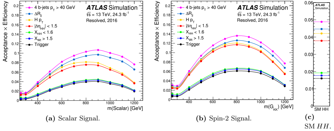
Figure 2. The selection acceptance times efficiency at each stage of the event selection for (a) a narrow-width scalar and (b) G_{KK} \rightarrow HH \rightarrow b\bar{b}b\bar{b} with k/\bar{M}_{P1} = 1 for a range of resonance masses and (c) the SM non-resonant signal. Each selection step is detailed in section 5.1.
