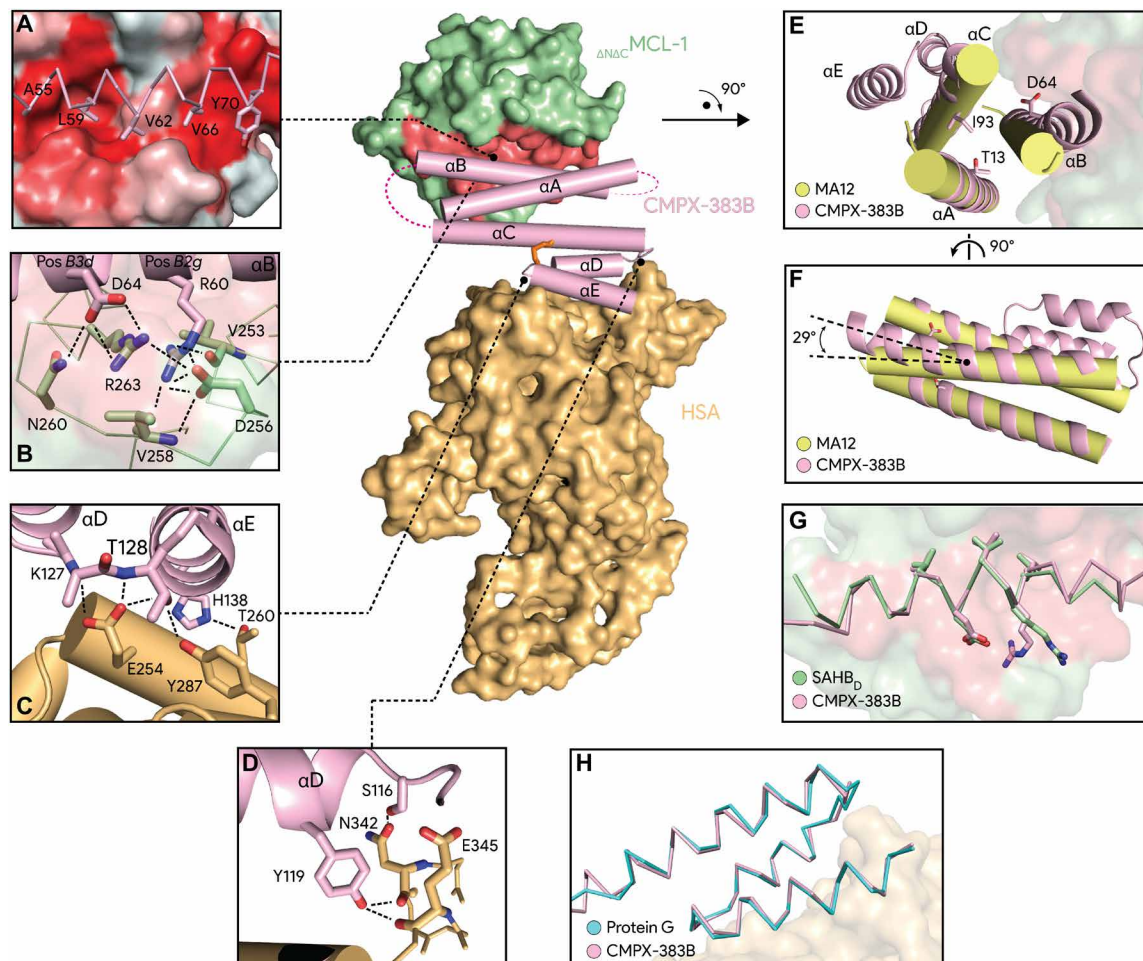
Fig. 6. Structural validation of the applied engineering strategies. Middle: Structural superposition of crystal structures featuring CMPX-383B (pink) in complex with either \Delta_{\text{NAC}} MCL-1 (green) or HSA (orange). Alphabody CMPX-383B is shown in cartoon representation. The linker regions between \alpha -helix A and B and between \alpha helices B and C are represented as dashed lines. The cysteine disulfide bridge that covalently links \alpha helices E to C (dark orange) is shown in stick representation. \Delta_{\text{NAC}} MCL-1 and HSA are shown in surface representation. The BH3-binding groove of \Delta_{\text{NAC}} MCL-1 is colored red. (A) Detailed view of the hydrophobic interface between \alpha helices B of CMPX-383B and the BH3-binding groove of \Delta_{\text{NAC}} MCL-1. \alpha Helix B of CMPX-383B is shown as ribbon diagram, and \Delta_{\text{NAC}} MCL-1 is shown in surface representation and colored according to the Eisenberg hydrophobicity scale (red is more hydrophobic). (B) Detailed view of the electrostatic interactions around Asp 64 and Arg 60 of CMPX-383B at the BH3-binding groove of \Delta_{\text{NAC}} MCL-1. (C and D) Detailed views on how CMPX-383B engages HSA using predominantly electrostatic interactions at \alpha helix D, the \alpha D- \alpha E loop, and \alpha helix E. (E and F) Structural superposition of CMPX-383B (pink; canonical helix representation) and the canonical IL-23 binding Alphabody MA12 (yellow; cylindrical helix presentation, generated using PDB code 5MJ3), highlighting the distinct arching of \alpha helix B of CMPX-383B allowing a full occupancy of the BH3-binding groove of \Delta_{\text{NAC}} MCL-1 (surface representation). (G) Structural superposition of the inhibitory MCL-1 helix SAHB D (green; PDB code 3MK8) with \alpha helix B of CMPX-383B (pink), both when in complex with MCL-1 (surface representation). (H) Structural superimposition of the albumin-binding moiety of F. magna protein G (cyan; generated using PDB code 1TF0) and \alpha helices C, D, and E of CMPX-383B (pink), both bound to HSA (orange; surface representation).
