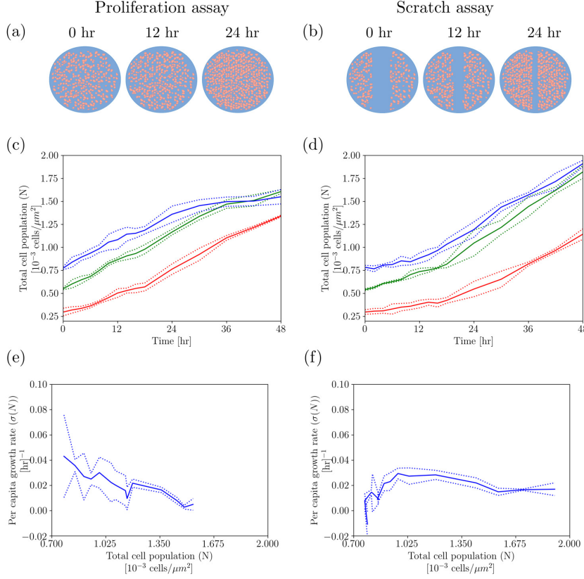
Fig. 1 Schematic representation of how the (a) proliferation and (b) scratch assays evolve in time. In the plots (c)-(f), we consider the experimental data from the proliferation and scratch assays performed in [24]. The authors consider three replicates for three initial degrees of confluence. In (c) and (d) the mean and the standard deviation of the cell population is plotted over the duration of the experiment for each initial degree of confluence. In (e) and (f) the mean and the standard deviation of the per capita growth rate \sigma(N) = \frac{dN}{dt} \frac{1}{N} is plotted with respect to the mean cell population N . For plots (e) and (f) we consider only the assays with the highest degree of confluence. We calculate the per capita growth rate in the same way as in [24]. A biphasic trend can be observed in (f) (for the scratch assay) but not in (e) (for the proliferation assay).
