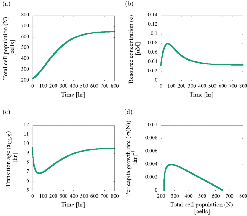
Fig. 2 Evolution of the age-structured model with resource-regulated proliferation, Eqs. (1) and (4). In (a) we plot the total cell population evolution and observe it follows a logistic-type growth. In (b) we plot the resource evolution that follows a rapid increase and then a monotonic decrease to the steady-state value. In (c) we plot the evolution of the transition age a_{G1/S}(t) and the inverse dependence of the resource concentration on the transition age can be observed. In (d) we plot the per capita growth rate against the total cell population evolution for which two proliferation phases can be observed (a rapid increase, then slower decrease). Parameter values as per Table 1.
