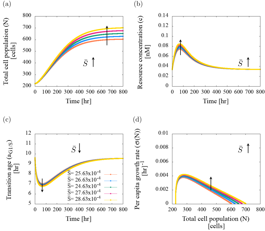
Fig. 3 Series of plots showing the dynamics of the coupled age-structured model with resource-regulated proliferation given by Eqs. (1) and (4), as we vary the resource flux, \bar{S} . Increasing the value of \bar{S} : (a) increases the steady-state value of the total cell population, N_\infty , (b) increases the maximum resource concentration and the time it takes to reach the steady-state value, and (c) reduces the minimum value of the transition age a_{G1/S} . (d) The plots of the per capita growth rate against the total cell population exhibit biphasic dynamics for the selected values of \bar{S} . Parameter values as per Table 1.
