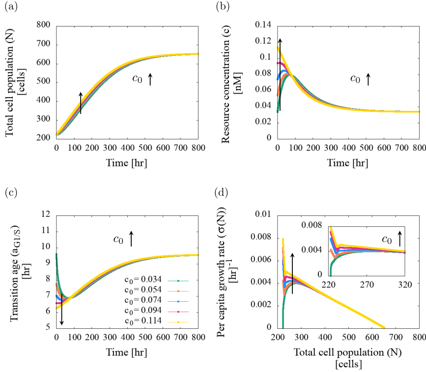
Fig. 4 Series of plots showing the dynamics of the coupled age-structured model with resource-regulated proliferation, given by Eqs. (1) and (4), as we vary the initial resource concentration value, c_0 . Increasing c_0 : (a) does not affect the total cell population, increases the maximum resource concentration but reduces the time it takes to reach it, and (c) makes the initial decrease of the transition age a_{G1/S} disappear. (d) Increasing the initial resource concentration, c_0 , affects the plots of the per capita growth rate against the total cell population by shortening the duration of the disturbance phase where there is no monotonic decreasing dependence. Parameter values as per Table 1.
