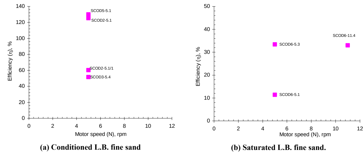
Figure 6.59. Discharge efficiency vs motor speed for L.B. fine sand tests.
