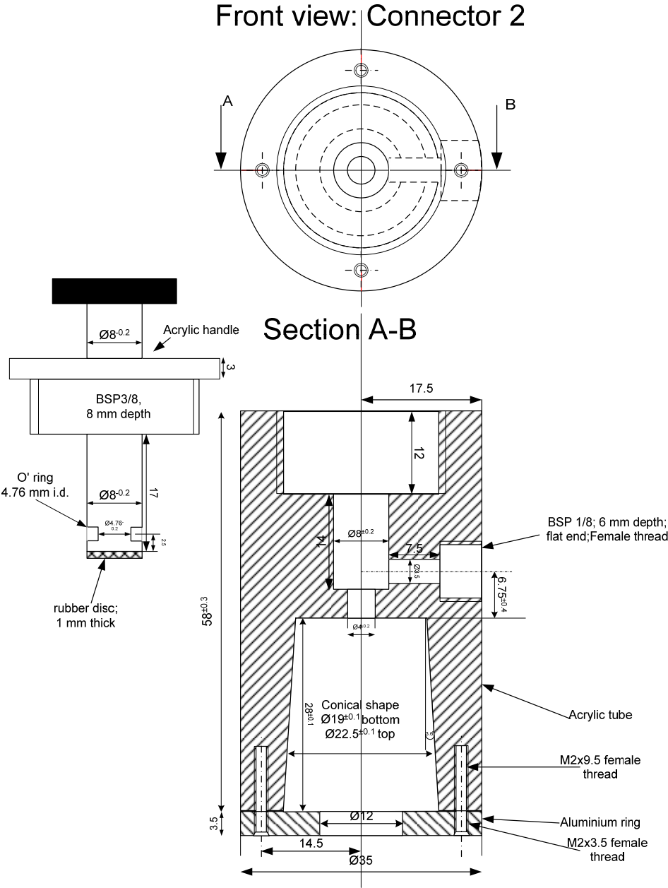
Figure 5.10. New capillary tube system: top connector (all units in millimetres).
