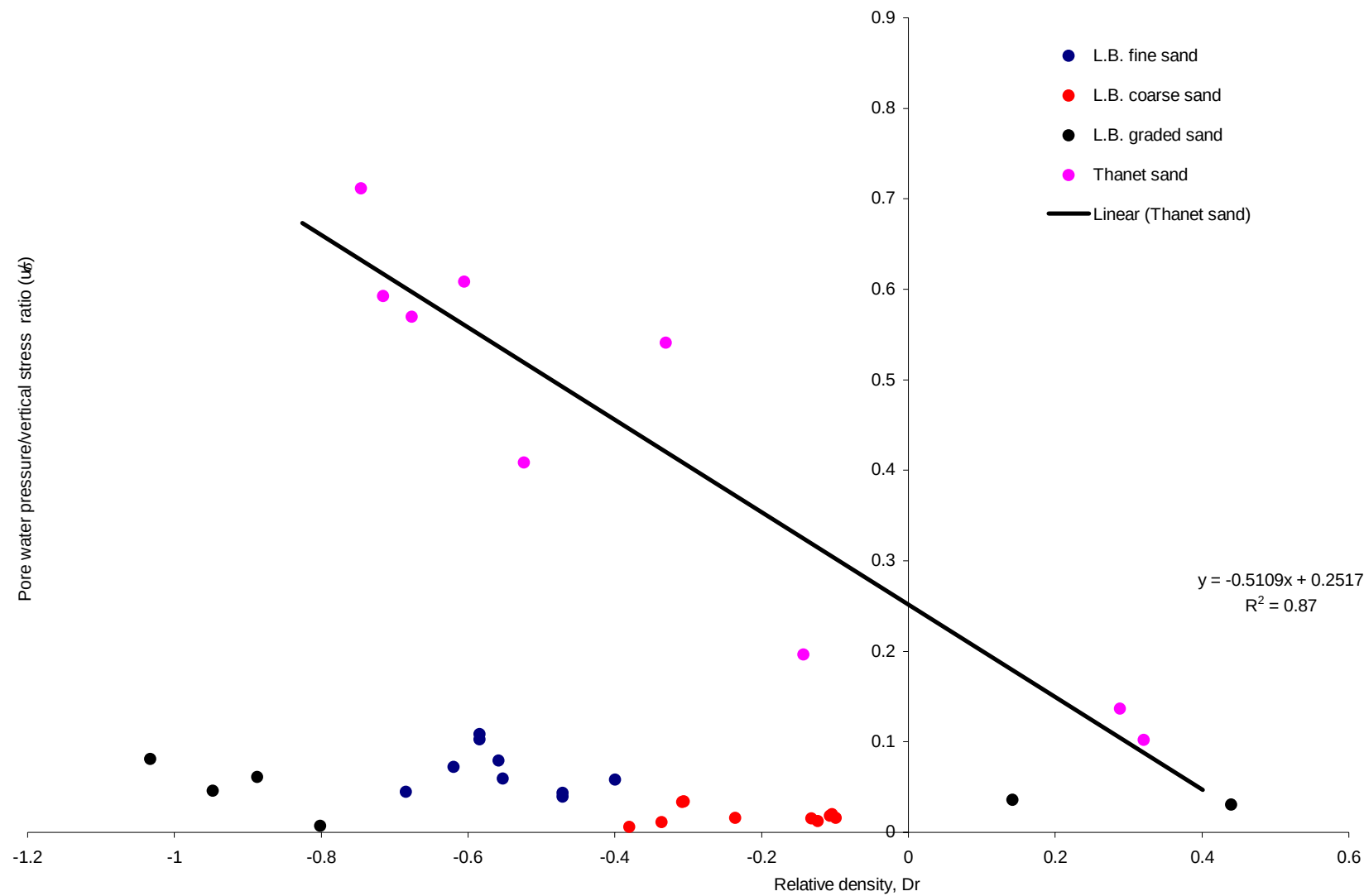
Figure 4.31. Variation of pore pressure/vertical stress ratio with Relative density at 12 (mm) of horizontal displacement through the shear box test (Tests with Condition “ok” plotted).
