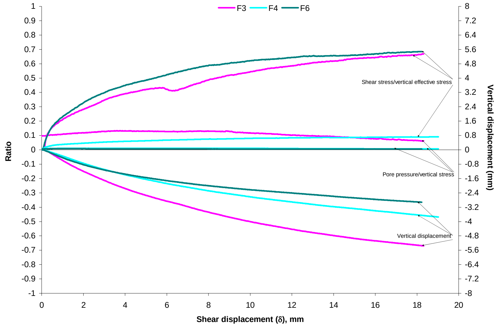
Figure 4.19. Shear stress/ vertical effective stress ratio, pore pressure/ vertical stress ratio and vertical displacement for tests F3, F4 and F6.
