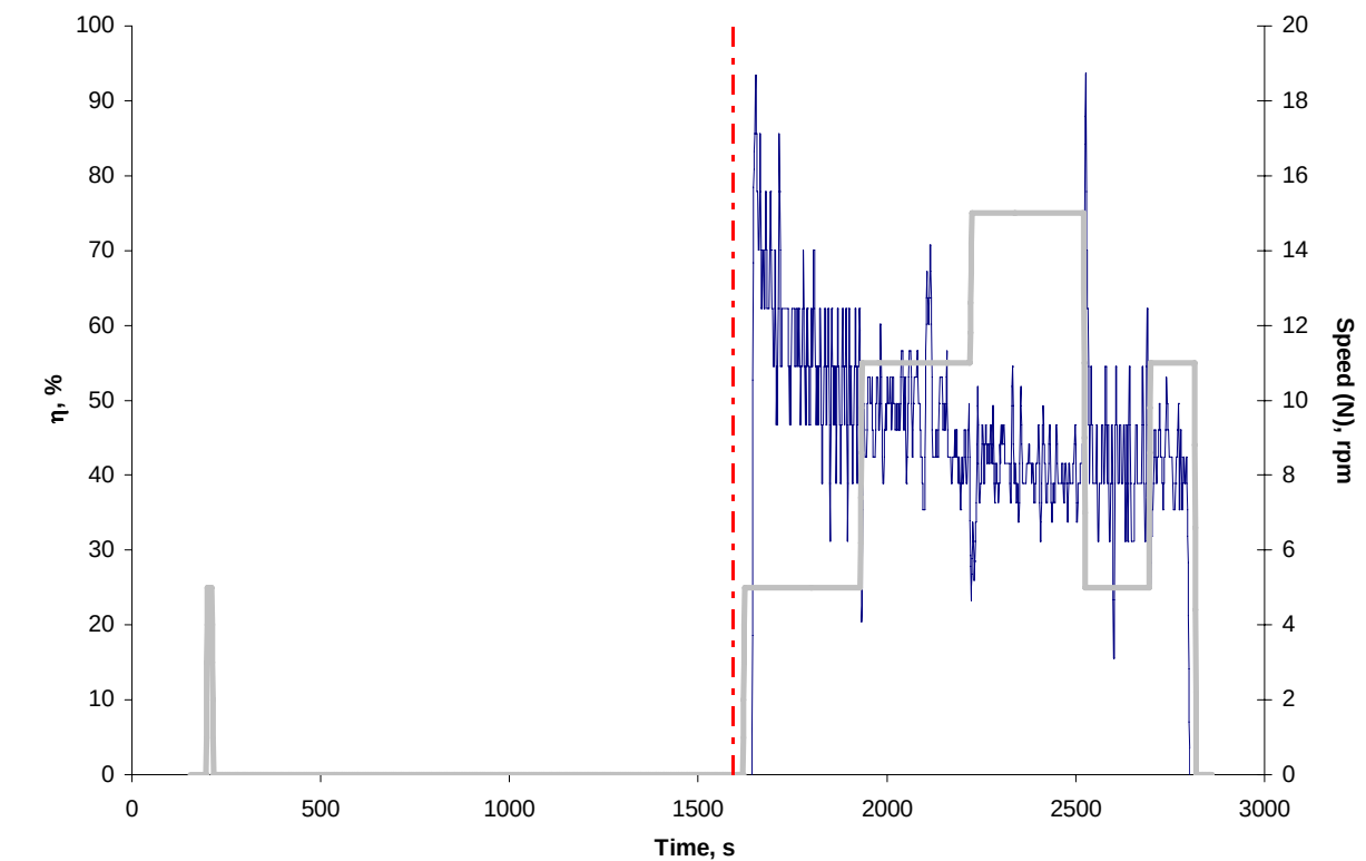
Figure 6.39. Efficiency for SCOD 9 test.
