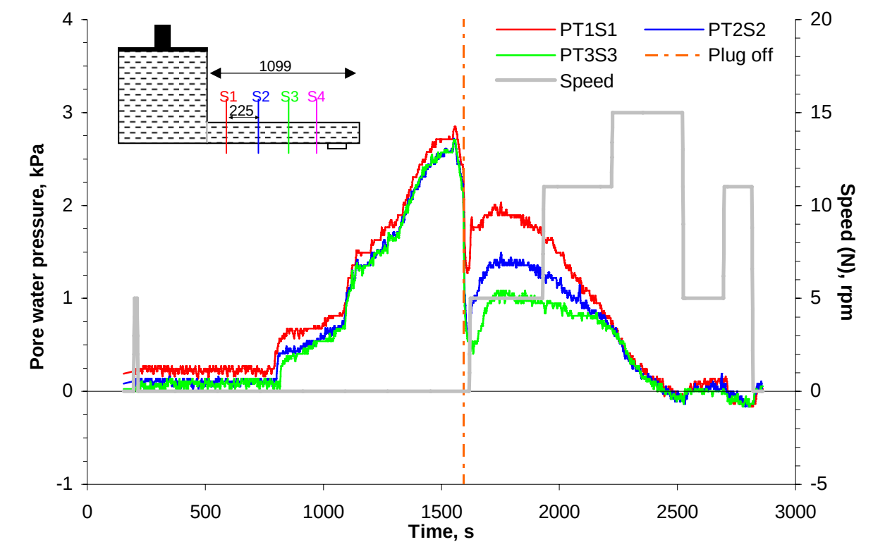
Figure 6.36. Pore water pressures measured for SCOD9 test.
