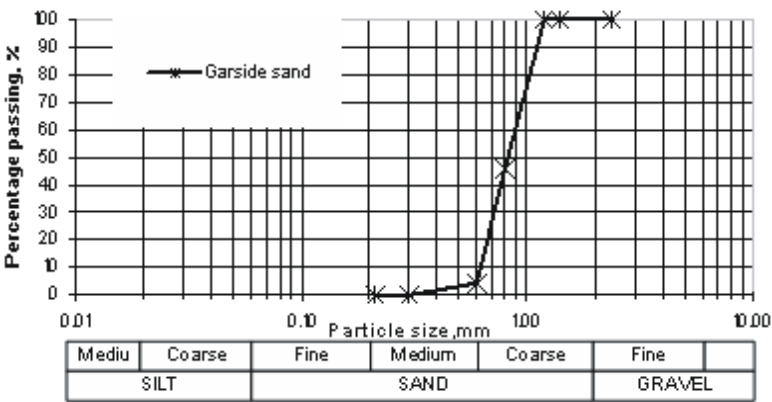
Figure 3.3. Grading curve of Garside sand.
