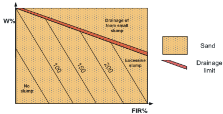
Figure 3.17. Slump variation on conditioned L.B. sands: (a) Slump vs FIR (b) w_{drum} vs FIR
