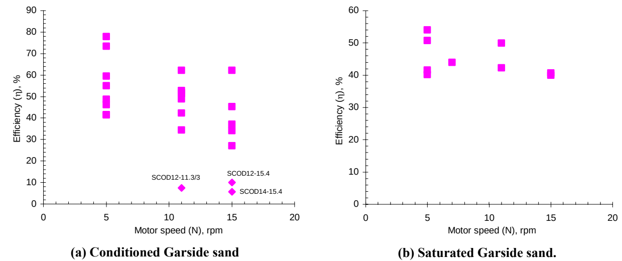
Figure 6.60. Discharge efficiency vs motor speed for Garside sand tests.
