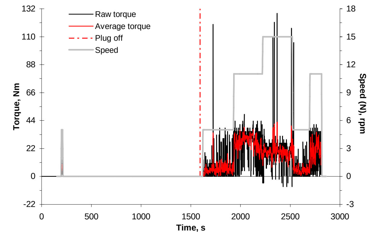
Figure 6.37. Torque calculated for SCOD 9 test.
