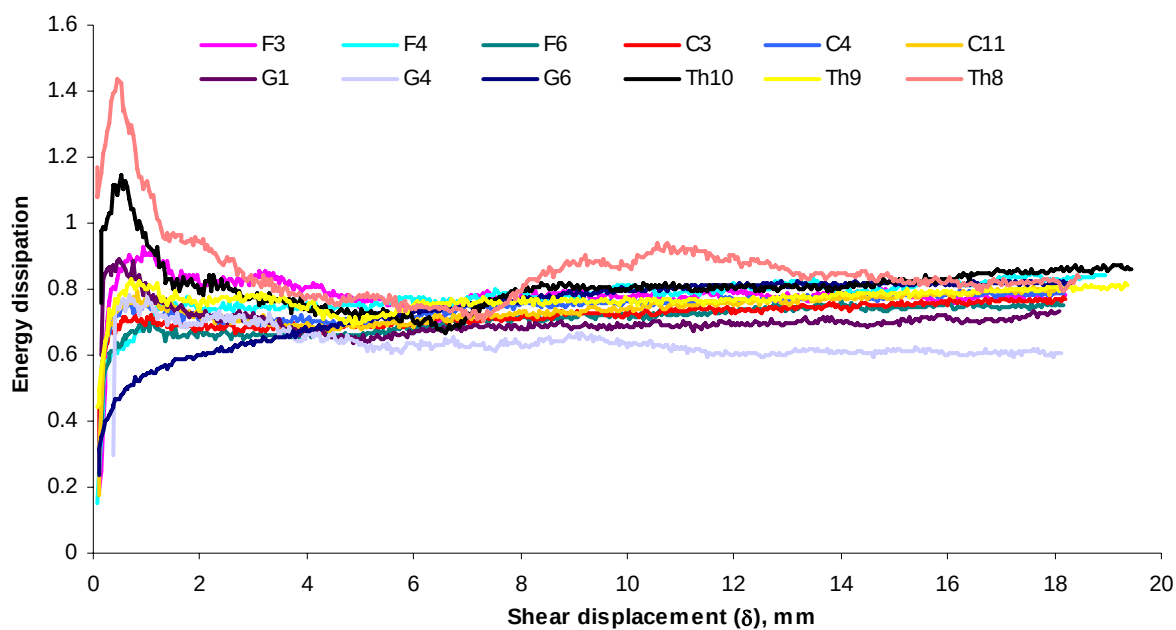
Figure 4.23. Energy dissipation for F3, F4, F6, C3, C4, C11, G1, G4, G6, Th8, Th9 and Th10.
