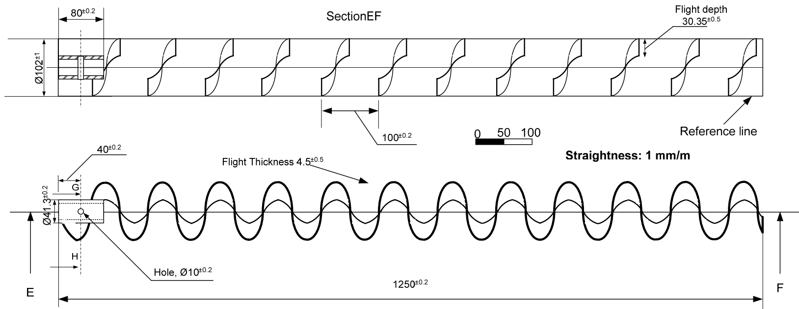
Figure 6.15. Screw without central shaft.
