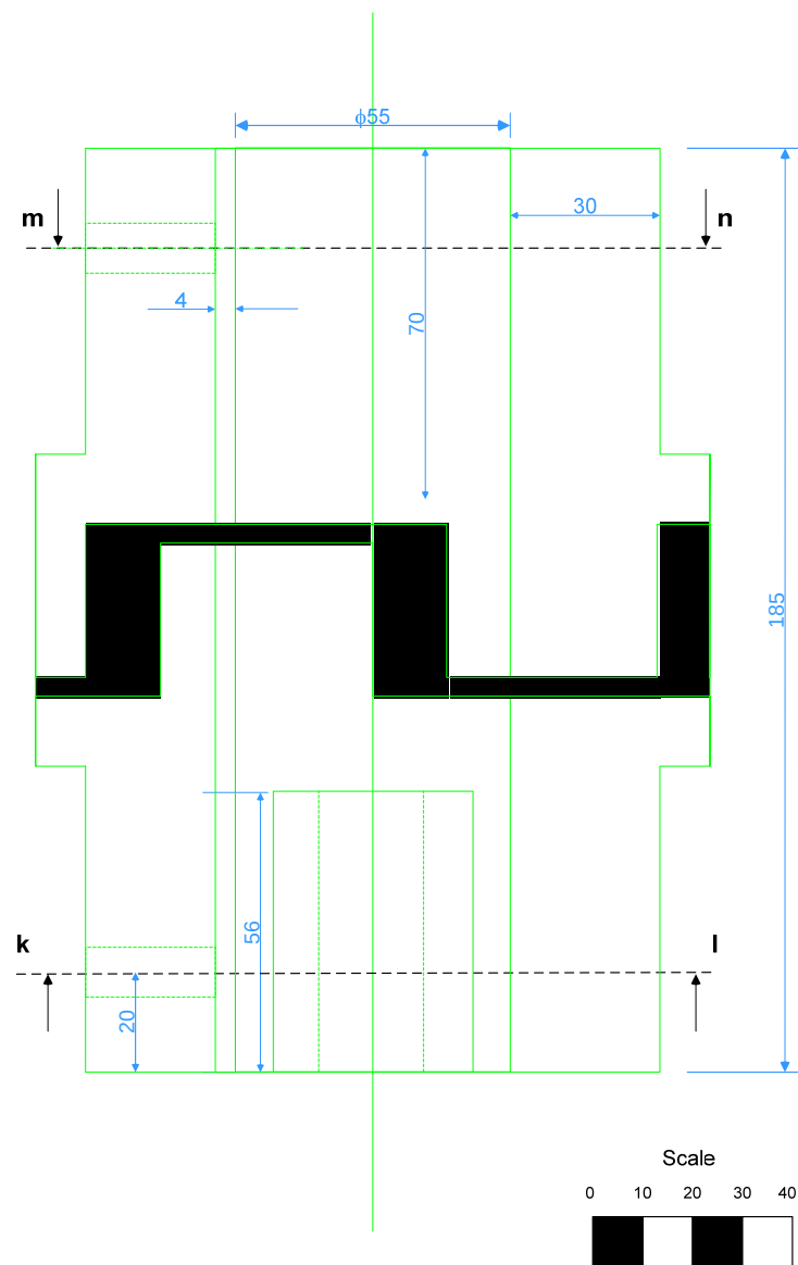
Figure 6.9. Torque coupling.
