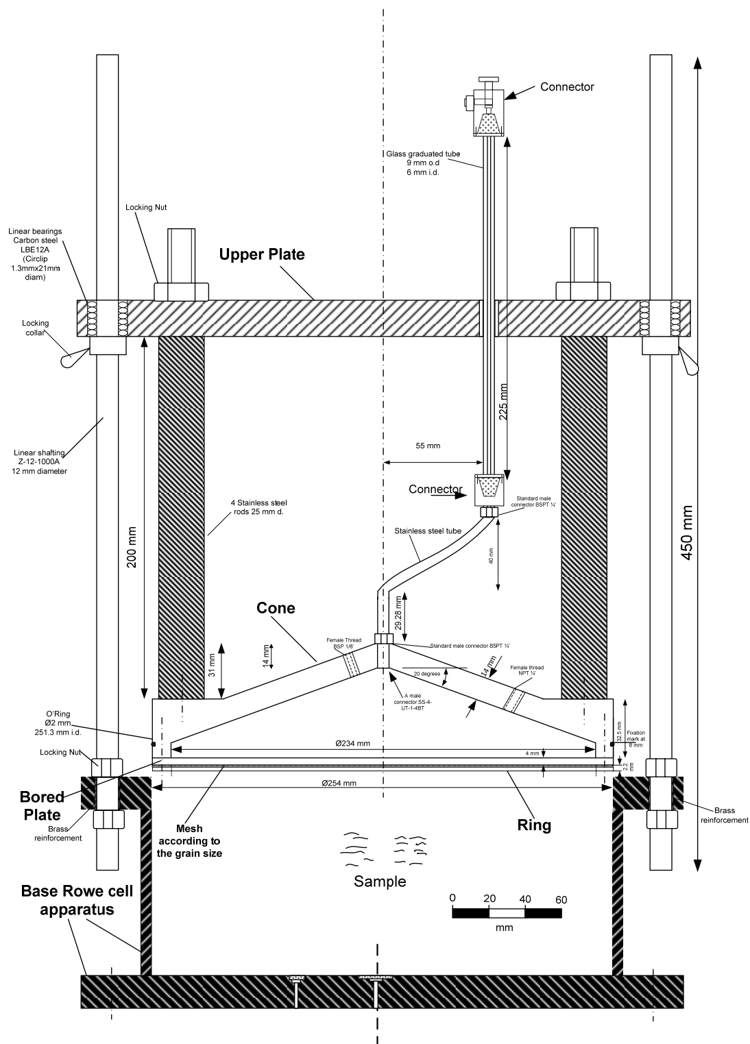
Figure 5.3. MAPC section.
