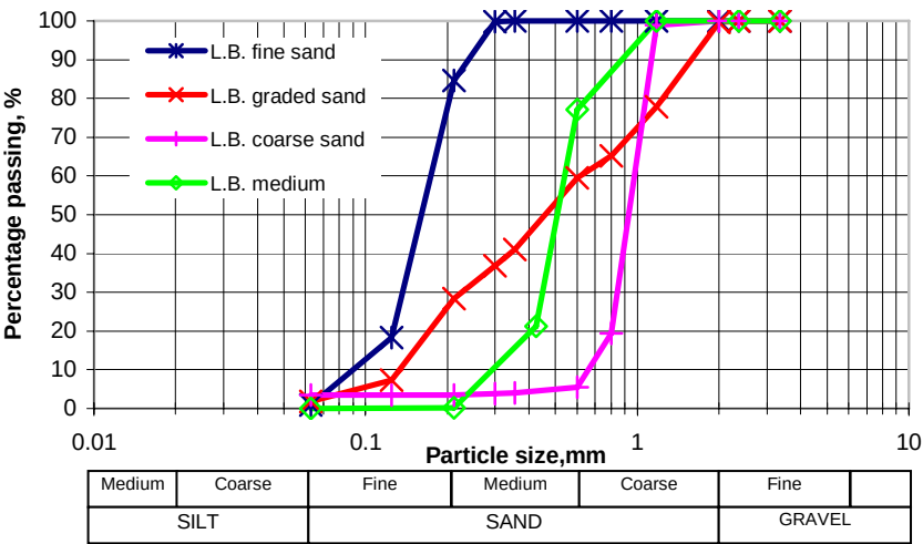
Figure 3.1. Grading curve of L.B. fine sand, L.B. coarse sand, L.B. graded sand and L.B. medium coarse sand.
