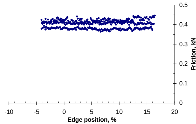
Figure 5.19. Friction- loading, displacement rate 5 mm/min-
