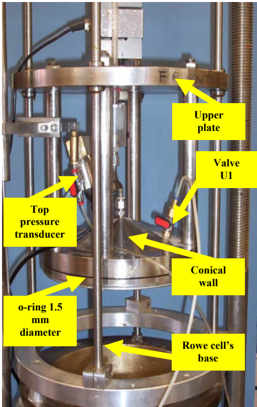
Figure 5.4. MAPC top view.
