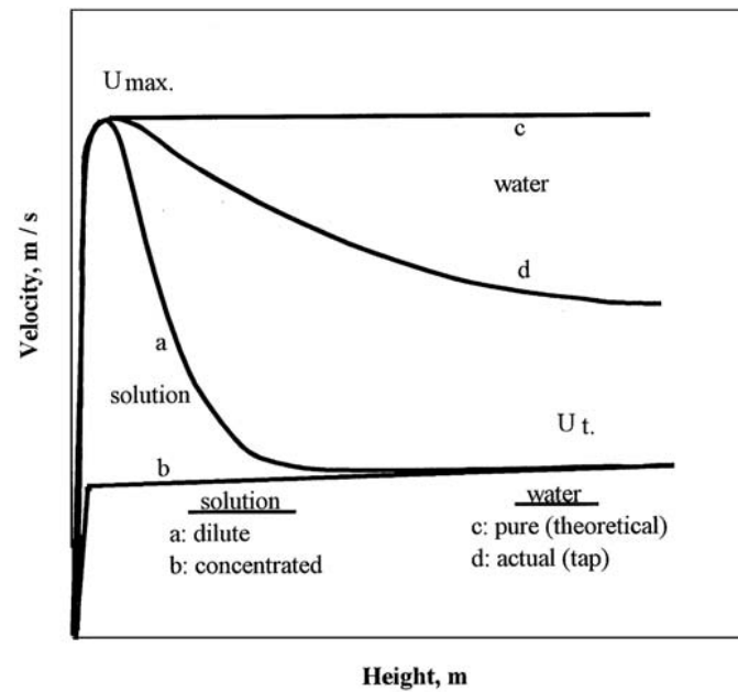
Figure 2.5. Typical bubble velocity profiles for a bubble rising in water and surfactant solution. Indicated are the maximum velocity ( U_{\max} ) and terminal
