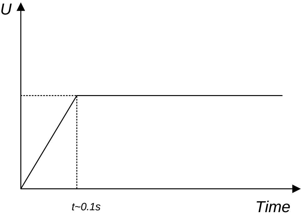
Figure 5.26. Terminal velocity of bubble.
