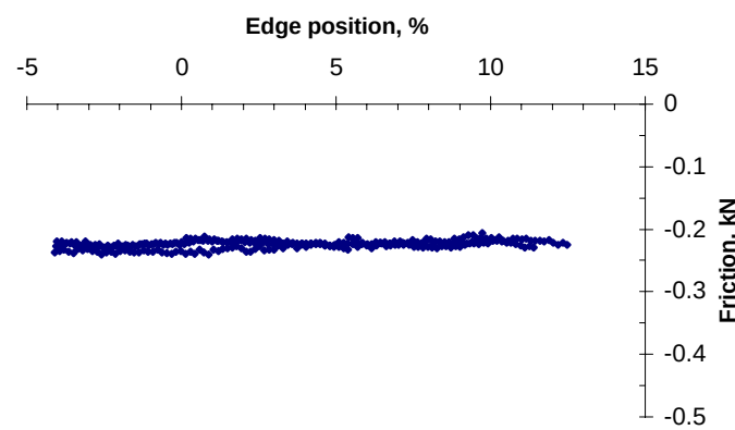
Figure 5.20. Friction- unloading, displacement rate 5 mm/min-
