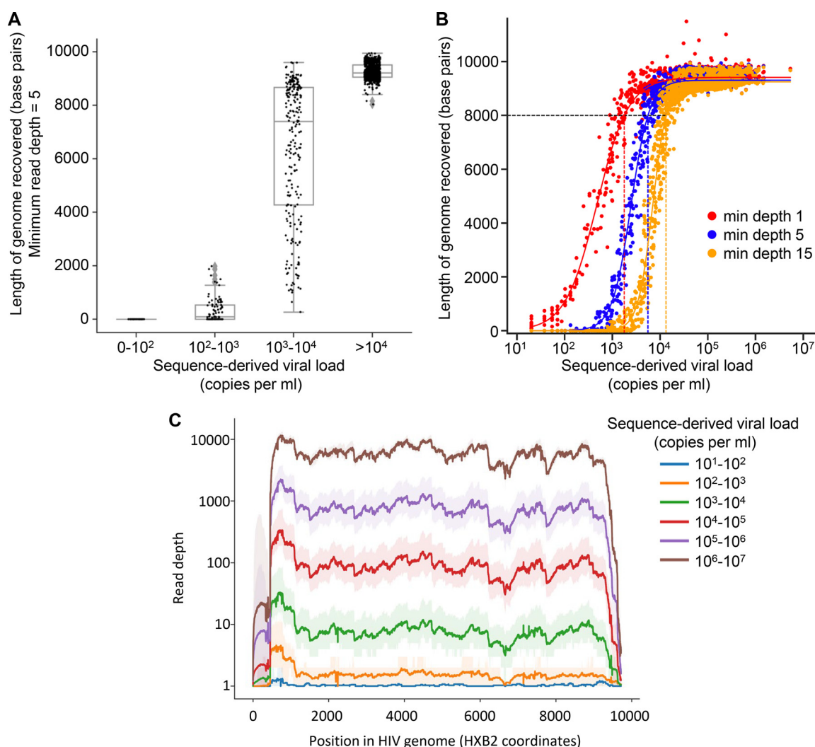
FIG 4 Sequencing success is influenced by viral load. (A) The length of the HIV genomes reconstructed by shiver software, from paired-end Illumina reads, stratified by log viral load, showed reproducible whole-genome coverage for samples with sequence inferred viral loads of >4 \log_{10} copies/ml and near-complete coverage for the majority of samples with VL between 3 and 4 \log_{10} copies/ml. (B) The viral loads at which genome coverage exceed 8 kb with minimum depth thresholds of 1 read, 5 reads, and 15 reads (after removal of PCR duplicates) are shown by the intercepts of curves fitted using a sigmoid function. (C) The median (thick lines) and 95th percentile range (ribbons) of read-depth observed across the genome are shown for all samples, grouped by sequence-derived viral load.
