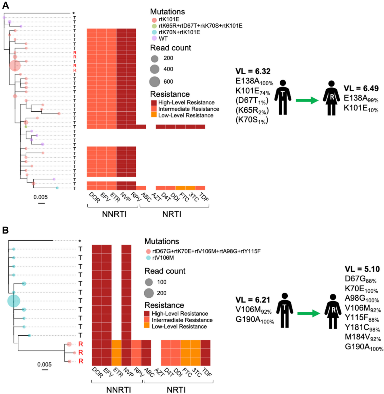
FIG 5 Within-host phylogenetic trees of Illumina reads spanning drug resistance sites in pol . Phyloscanner software performs ancestral state reconstructions of phylogenetic trees generated from Illumina reads in “windows” across the genome in order to identify pairs consisting of transmitters (T) and recipients (R). Phylogenetic trees of reads spanning drug resistance mutations sites in pol are shown for two inferred transmission pairs (A and B). Tree tips (circles) are colored by the combinations of drug resistance mutations observed for each unique taxon and scaled to total read counts within each taxa (after removal of PCR duplicates). Heatmaps report the predicted drug susceptibilities for each read using the Stanford HIVdb classification. Sequence-derived viral loads (log 10 RNA copies/ml) and the complete list of resistance mutations with associated frequencies, observed across entire genomes, are shown for each individual. Mutations observed at frequencies below 5% are shown in parentheses.
