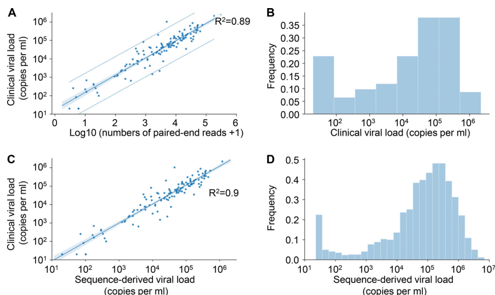
FIG 2 Viral load is calculated from the number of sequencing reads. (A) The data and linear regression model estimates for the viral load standards. The narrow shaded area is the 95% confidence interval for the regression curve, and the dashed lines are 95% prediction intervals for measurements. The mean squared error of prediction was 0.324 \log_{10} copies/ml. (B) Distribution of independently measured clinical viral loads in a subset of 146 samples used to assess model performance. (C) Relationship between the clinical viral load and the sequence-derived viral load from the model shown in panel A for these 146 samples. (D) Frequency of sequence-derived viral load estimates for all 1,620 samples.
