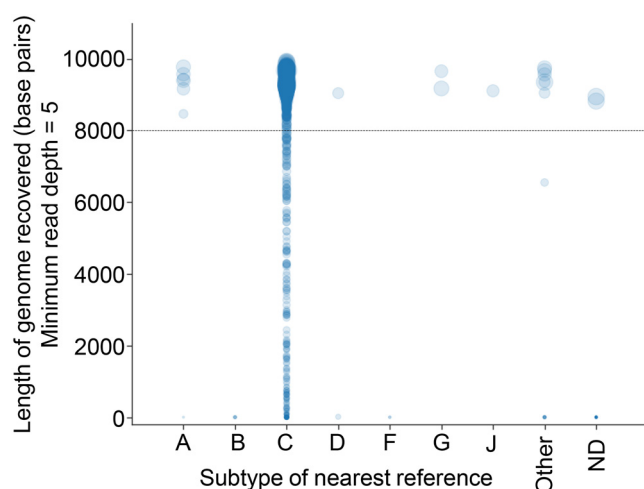
FIG 3 veSEQ-HIV is both sensitive and specific. Figure shows the length of recovered HIV genome for all sequenced samples. We consider a position in the genome to be accurately determined when the read depth is at least five. The category “Other” consists of potential intersubtype recombinants. Quantitative standards (HXB2, subtype B) are included in all sequencing runs, but are not displayed in this analysis.
