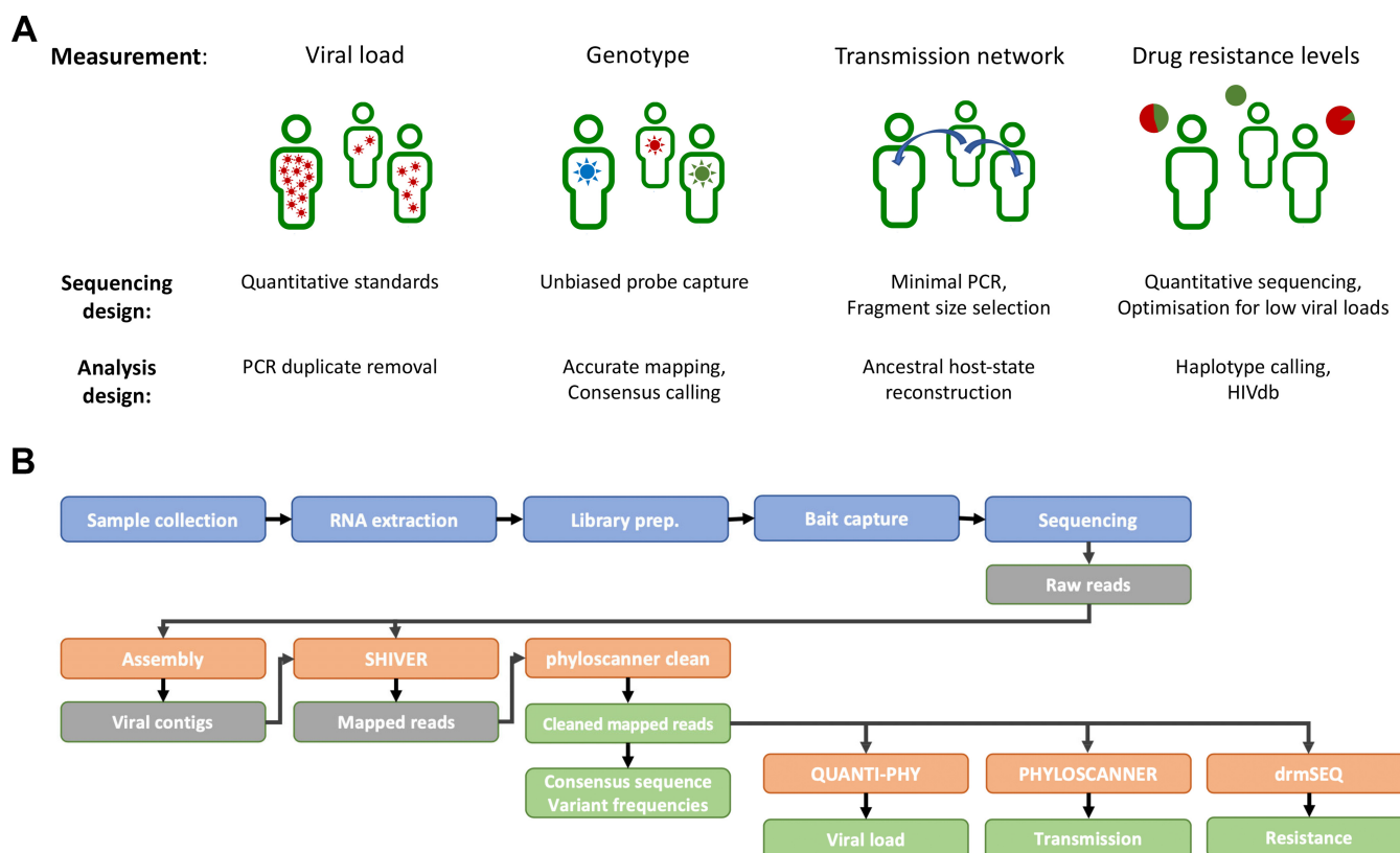
FIG 1 veSEQ-HIV includes a sequencing protocol and bioinformatics pipeline, yielding information on individual and population levels. (A) The veSEQ-HIV method was developed to provide multiple measurements from a single assay, including viral load, HIV genotype, drug resistance, and transmission inference. (B) Overview of veSEQ-HIV: a complete laboratory and computational pipeline for high-throughput sequencing. RNA extraction from plasma samples is carried out in a CL-3 certified laboratory, before transfer to a dedicated genomics facility for library preparation, bait capture, and finally sequencing. Raw sequencing data are preprocessed to remove host and contaminant RNA, and these computationally filtered reads together with their de novo -assembled contigs are used to determine the consensus genome and minority variant frequencies using shiver . QC metrics are then calculated, and the proportion of contaminant reads originating from other samples is estimated with Kallisto. Samples which result in a successful read mapping are then cleaned with phyloscanner to remove contaminant reads, and clean reads are used to infer transmission patterns with phyloscanner , and to make drug resistance predictions with HIVdb and drmmSEQ .
