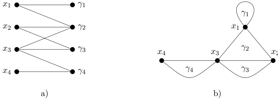
Figure 1: Graphs from Example 1.
