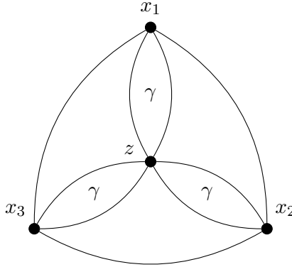
Figure 2: Instance from Example 2.
