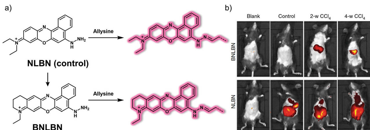
Fig. 24 (a) Chemical structure of the small molecule-based NIR probes NLBN (control) and BNLBN and working model for how the latter may be used to detect allylsine. (b) In vivo fluorescence images of mice in the blank, normal, 2-w CCl 4 and 4-w CCl 4 groups recorded after subjecting to NLBN (100 μL, 200 μM, i.v. injection) and BNLBN (100 μL, 200 μM, i.v. injection). Blank: without any treatment; control: treated with PBS; mild fibrosis: twice a week, intraperitoneal injection of CCl 4 (10% in olive oil; 1 mL kg -1 , for 2 weeks); severe fibrosis: the same treatment but for 4 weeks. Reproduced with permission from ref. 34. Copyright (2020) by the authors (P. Xing, Y. Niu, R. Mu, Z. Wang, D. Xie, H. Li, L. Dong and C. Wang). Published by Springer Nature.
