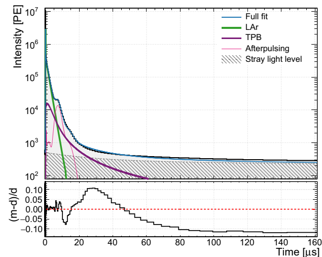
Fig. 5 At time scales beyond 15 \mu s , the pulseshape is dominated by the delayed TPB emission. At approximately 30 \mu s , the intensity of TPB emission has declined to the point where it is equal to the intensity of left-over late light from previous events
