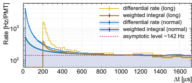
Fig. 3 The pre-event light level as a function of \Delta t , for normal (16 \mu\text{s} ) and long (200 \mu\text{s} ) PMT trace data. Both the differential rate, and the average light level above the \Delta t value (see text) are shown. In all cases, the curves approach a light level of approximately 142 Hz. The peaks at 20 \mu\text{s} and 200 \mu\text{s} are due to pile-up (see text)
