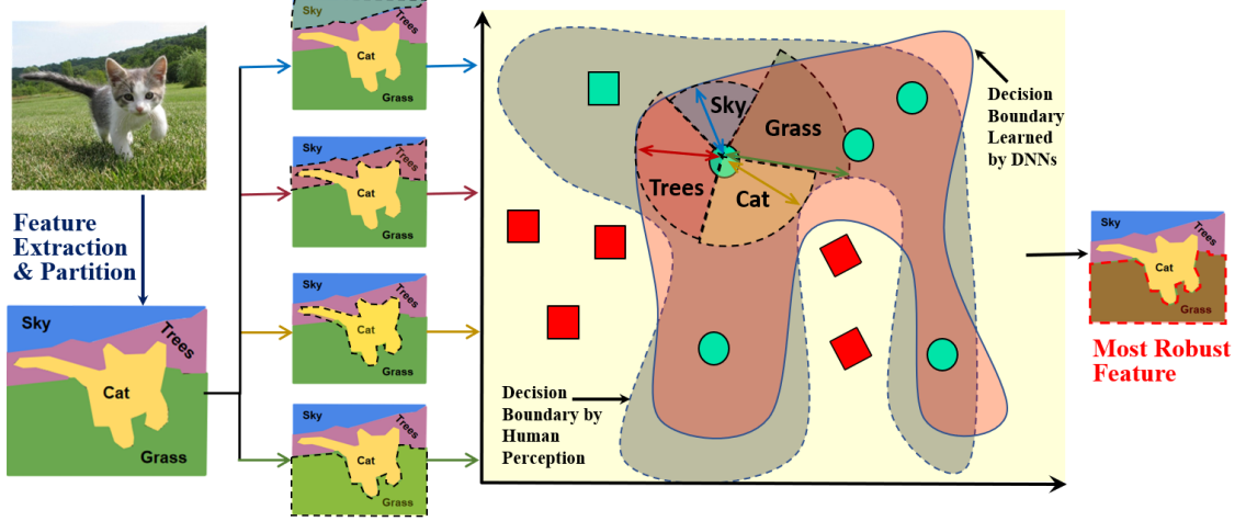
Figure 5.2: Illustration of the feature robustness ( \text{FR}_\Lambda ) problem, which aims to find, on an original image \alpha , a feature, or a subset of features, that is the most robust against adversarial perturbations. Given a benign image, we first apply feature extraction or semantic partitioning methods to produce a set of disjoint features (‘Sky’, ‘Trees’, ‘Cat’, etc.), then we find a set of robust features that is most resilient to adversarial perturbations (‘Grass’ in the figure), which quantifies the most robust direction in a safe norm ball.
