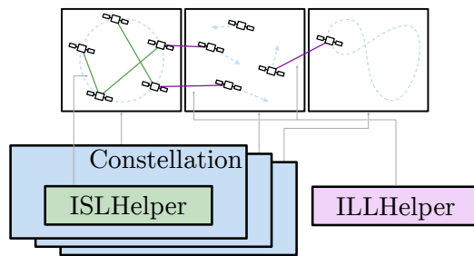
Fig. 6. DSNS can be extended to support new mobility and connectivity models by building new instances of the Constellation, ISLHelper, and ILLHelper classes.
