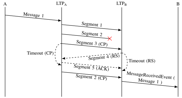
Fig. 3. Sequence diagram for LTP message retransmission. Segment 2 is lost in-transit and retransmitted to guarantee the message reaches its destination.
