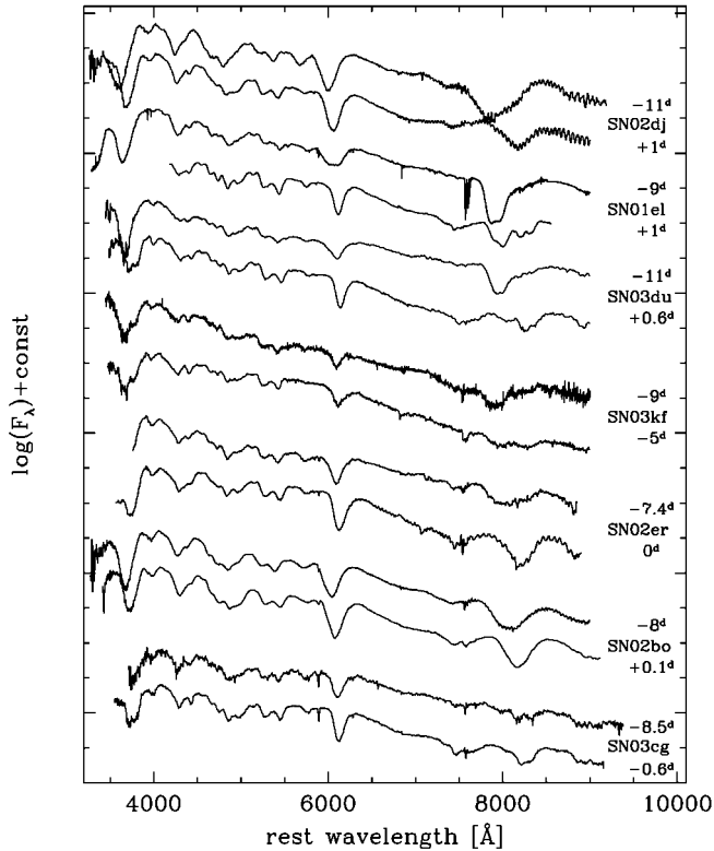
FIG. 1.—Spectra of the SNe Ia observed by the RTN: for each SN, the earliest spectrum is shown, together with a spectrum near maximum. The spectra have been corrected for reddening, arbitrarily scaled in flux, and are ordered by line velocity. Atmospheric absorption was removed from all spectra except those of SN 2001el.
