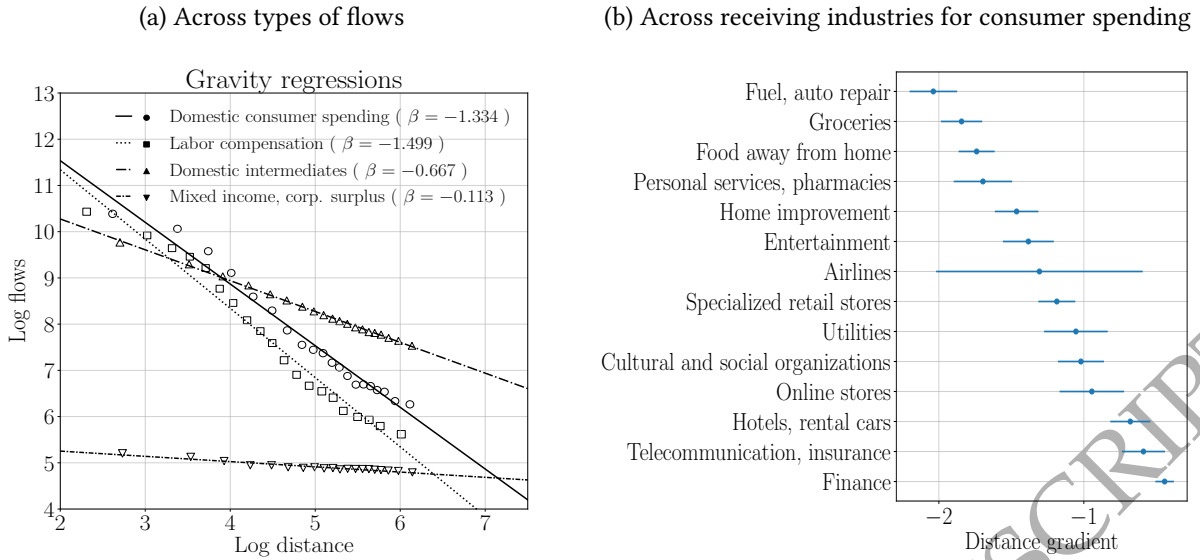
Figure V: Gravity equations
