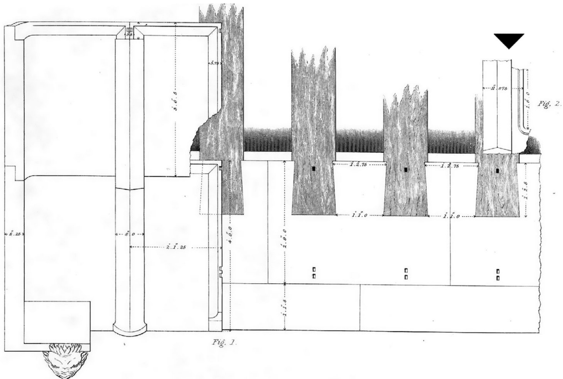
Fig. 9. Drawing showing the architectural roof structure of marble slabs in the roof tiles of the Parthenon. The arrow shows the opaia . Image: Cockerell 1860, pl. VII:2.
