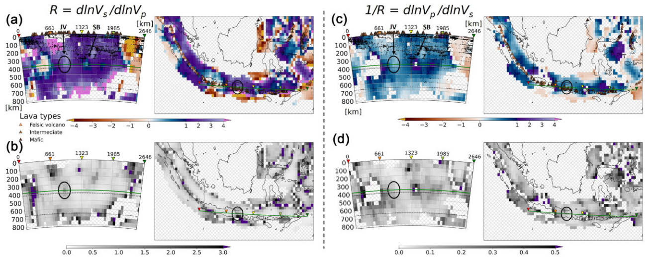
Figure 8. Same as Figs 7(b)–(f), but showing the d\ln V_s/d\ln V_p (a, b) and d\ln V_p/d\ln V_s (c, d) ratios.
