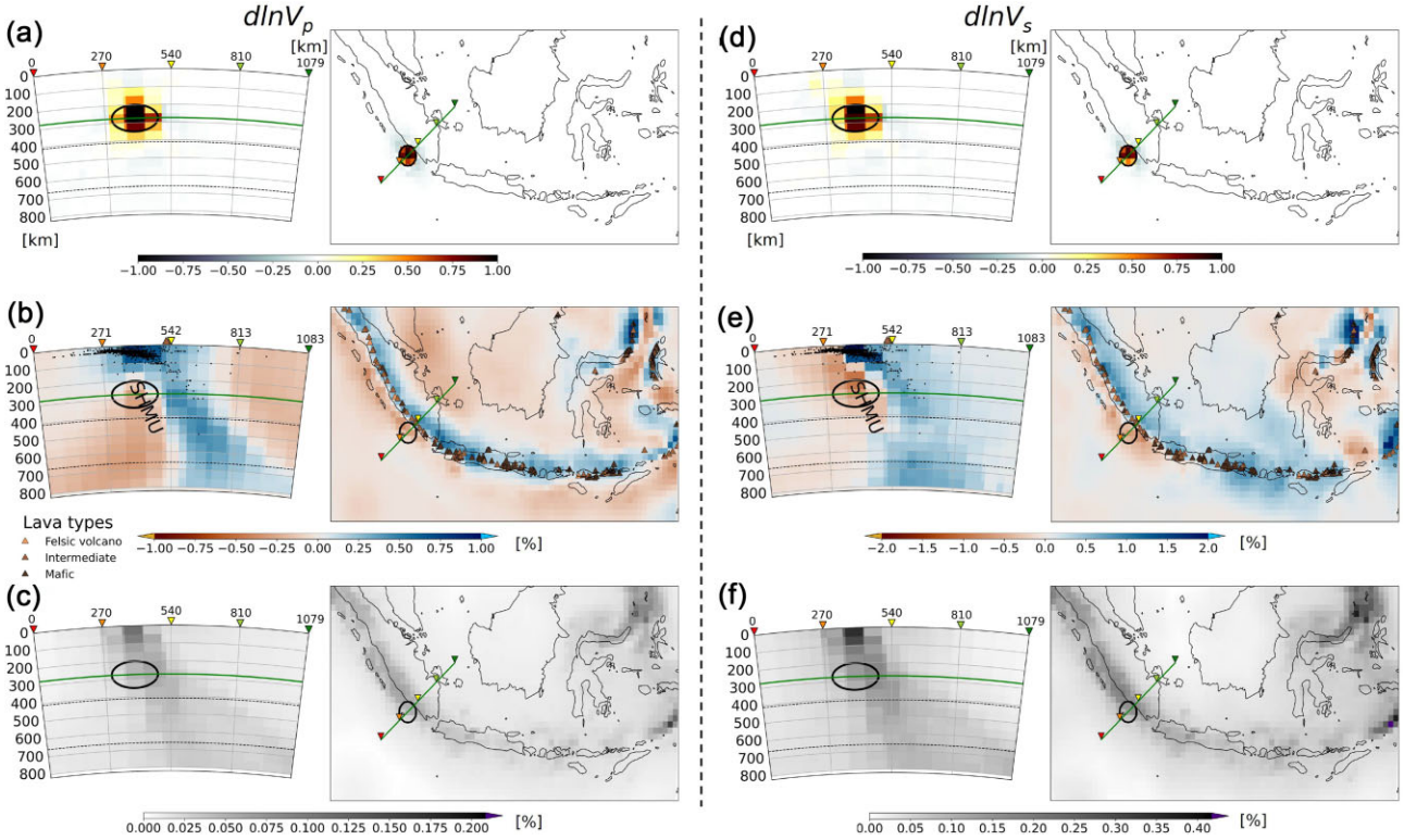
Figure 9. The region of the subslab negative velocity anomaly (SHMU), shown for both the d\ln V_p model (b, c) and the d\ln V_s model (e, f). An averaging kernel for the location of the SHMU is also shown (a, d), with the spatial extent of the target kernel indicated on all maps. For more details, see the caption of Fig. 7
