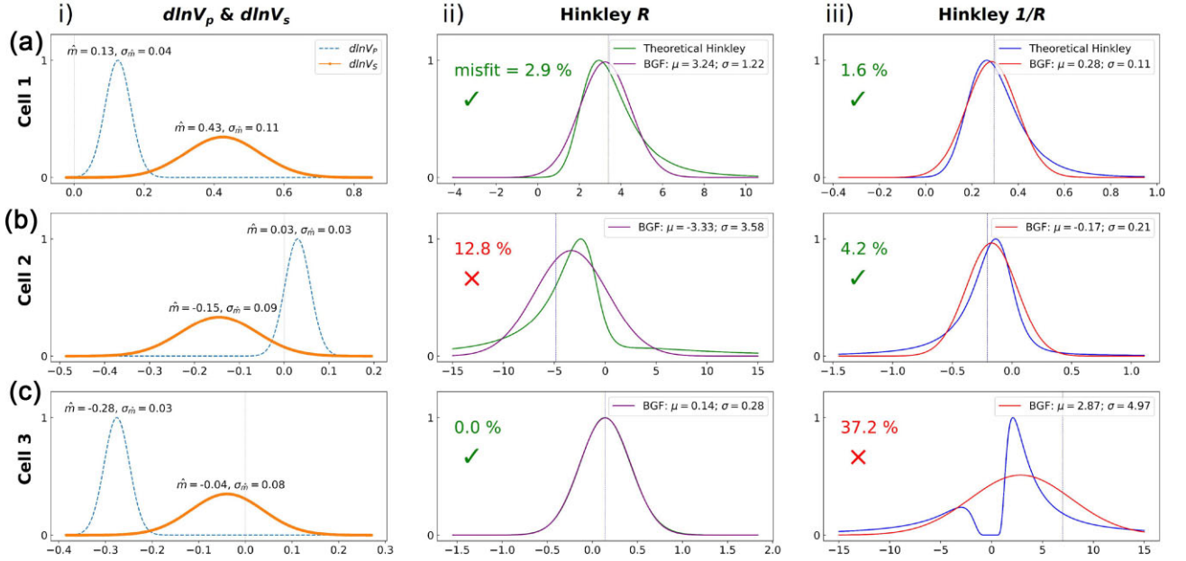
Figure 4. Examples of the Hinkley distributions for three different cells (a,b,c). For each example, we show: (i) the d\ln V_p (dotted blue) and d\ln V_s (orange) SOLA distributions; (ii) the d\ln V_s/d\ln V_p Hinkley distribution (green) and its best-fitting Gaussian function (BGF, here in purple) and (iii) the d\ln V_p/d\ln V_s Hinkley distribution (blue) with its BGF (red). In the top example, both ratios are considered Gaussian; in the middle, only d\ln V_p/d\ln V_s and in the bottom example, only d\ln V_s/d\ln V_p is Gaussian. In panels of R and 1/R , we also indicate the misfit between the Hinkley distribution and the BGF defined in eq. (10).
