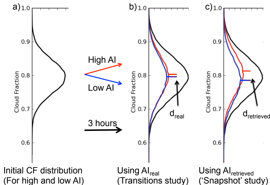
Fig. 8. Schematic demonstrating how the time of the aerosol retrieval can affect d(\text{CF}) . At the start of the timestep (a), both the high and low AI populations have the same CF distribution. (b) Despite starting with the same CF, these populations evolve differently, generating d_{\text{real}}(\text{CF}) at the end of the timestep. (c) Using the AI retrieval from the end of the timestep ( \text{AI}_{\text{retrieved}} ) gives a larger CF difference d_{\text{retrieved}}(\text{CF}) , due to contamination effects from relative humidity and cloud contamination which increase with CF.
