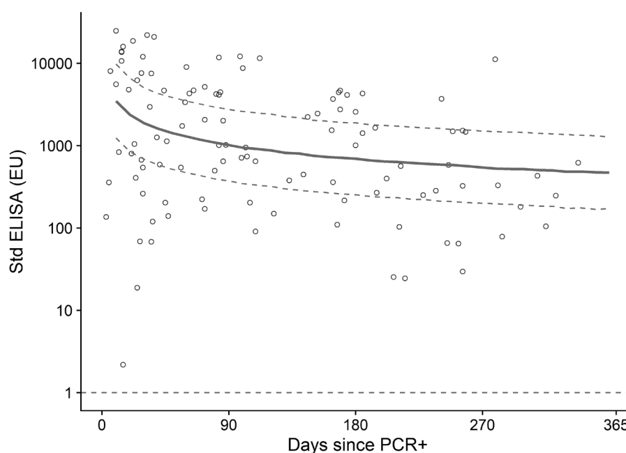
Figure 5. Anti-spike IgG by standardized ELISA in participants who were vaccinated and then had a positive PCR test. Data shown are ELISA values at timepoints after a positive PCR test, in participants who received two doses of vaccine prior to a positive PCR test. Each dot represents one sample. The solid line is the regression curve from a linear mixed model of log-transformed ELISA values regressed on log-transformed days since PCR test, with a participant-level random effect. Dotted curves show the bootstrapped predicted 95% confidence limits. Dotted horizontal line shows lower limit of the assay (EU=1)
