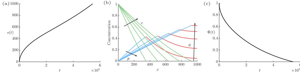
FIG. 4. (Colour online) Numerical results for the system (12)–(15) using the parameter values \beta = D_\phi = D_p = K = 1 , and d = 10^3 . (a) The position of the moving boundary, s(t) . (b) The concentrations of the cleanser, c (green), product in aqueous phase, p (blue), and product in oily phase, \phi (red), at times t = 1 \times 10^5, 2 \times 10^5, 3 \times 10^5, 4 \times 10^5, 5 \times 10^5 , where the arrows denote increasing time. (c) The proportion of remaining contaminant in the system, \Phi(t) , defined in (20a).
