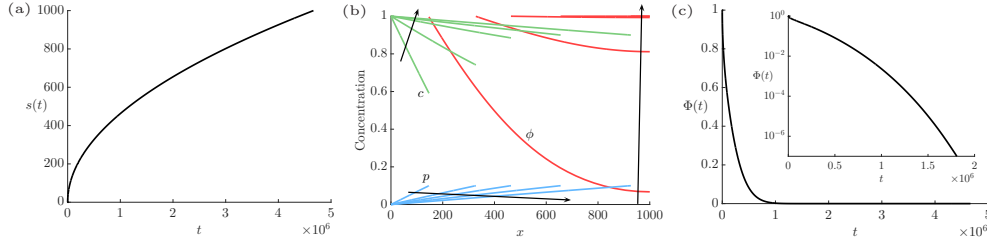
FIG. 3. (Colour online) Numerical results for the system (12)–(15) using the parameter values \beta = D_\phi = D_p = 1 , K = 10 , and d = 10^3 . (a) The position of the moving boundary, s(t) . (b) The concentrations of the cleanser, c (green), product in aqueous phase, p (blue), and product in oily phase, \phi (red), at (non-uniform) times t = 1 \times 10^5, 5 \times 10^5, 1 \times 10^6, 2 \times 10^6, 4 \times 10^6 , where the arrows denote increasing time. (c) The proportion of remaining contaminant in the system, \Phi(t) , defined in (20a). The inset shows a log-lin version of the same function.
