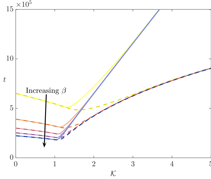
FIG. 5. (Colour online) The final time t_f (solid lines) and effective removal time t_e (dashed) as functions of K , calculated using numerical solutions of (12)–(15). Each line denotes a different value of \beta , corresponding to \beta = 1, 2, 3, 4 , and 5 . We use parameter values D_\phi = D_p = 1 , and d = 10^3 .
