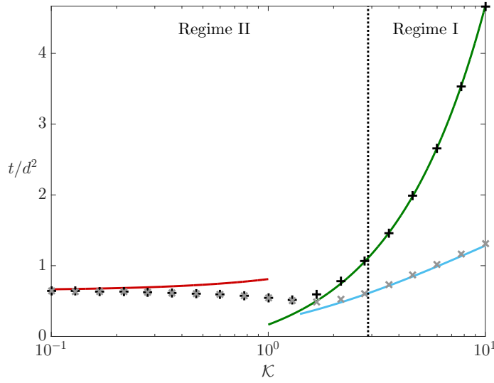
FIG. 9. (Colour online) The scaled final time t_f/d^2 and effective removal time t_e/d^2 as functions of K for \beta = D_\phi = D_p = 1 and d = 10^3 . The black addition signs are the numerically determined final times and the grey multiplication signs are the numerically determined effective removal times, both from the full problem defined in (12)–(15). For large K , we plot asymptotic approximations of t_f/d^2 (green) and t_e/d^2 (blue), from (44) and (47), respectively. For small K , the final and effective removal times coincide, and we approximate both with the red line using (28). The vertical black dotted line at K = 2.885 denotes the position of the critical line between regimes, defined by (41).
