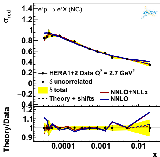
Fig. 10 The HERA NC E_p = 920 GeV data at Q^2 = 2.7 GeV 2 compared to the fits with and without \ln(1/x) resummation including this bin
