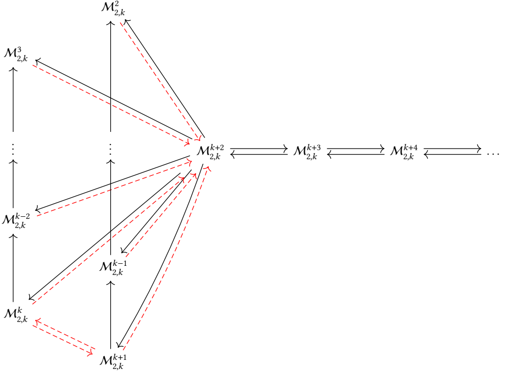
Fig. 2. Minions from Theorems 5.4, 5.17, 5.19, and 5.20. Solid black arrows indicate the existence of minion homomorphisms, whereas red dashed arrows indicate the non-existence of minion homomorphisms. We have taken the case when k is odd; if k is even, then \mathcal{M}_{2,k}^2 and \mathcal{M}_{2,k}^3 are swapped.
