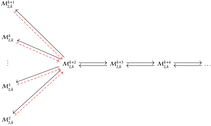
Fig. 1. Minions from Theorem 5.4. Solid black arrows indicate the existence of minion homomorphisms, whereas red dashed arrows indicate the non-existence of minion homomorphisms.
