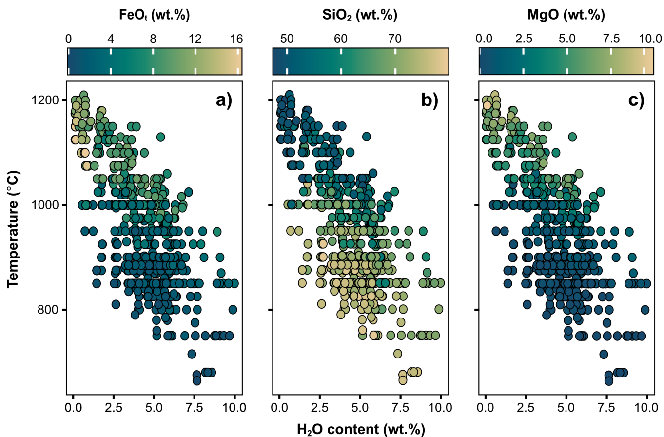
Figure S4. Temperature vs. H 2 O (wt.%) of experimental glass compositions with colour coding showing the (a) FeO t (wt.%), (b) SiO 2 (wt.%), and (c) MgO (wt.%) contents in the liquid. Note that all anhydrous experiments were removed.
