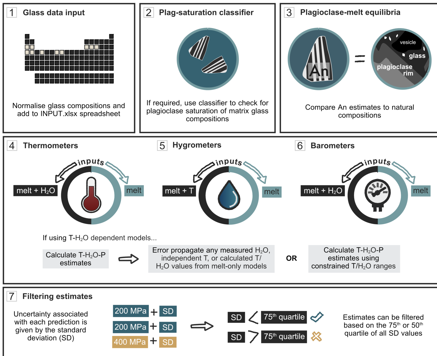
Figure S6. Schematic of recommended workflow to use the plagioclase-saturated melt models.
