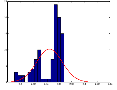
(f) Log-Normal and Translog
