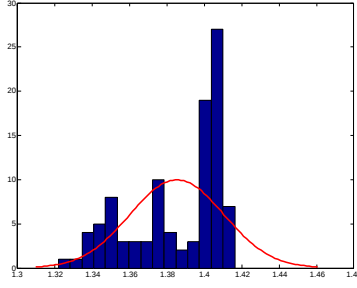
(b) Pareto and Linear
