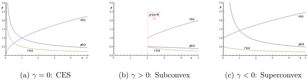
Figure 2: Examples of CREMR Demand Functions
