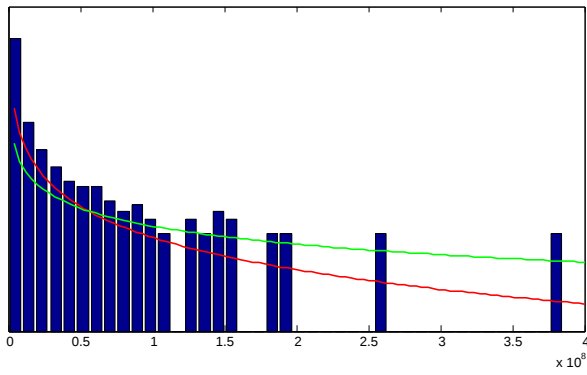
(a) Pareto and Log-Normal
