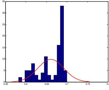
(e) Log-Normal and Linear
