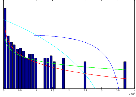
(b) Linear Demand with Pareto and Log-Normal
