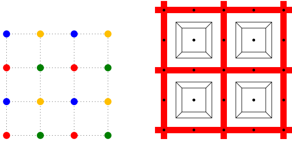
Figure 4: Left: the division of the grid into four sets. Right: one of the four g_i functions.
