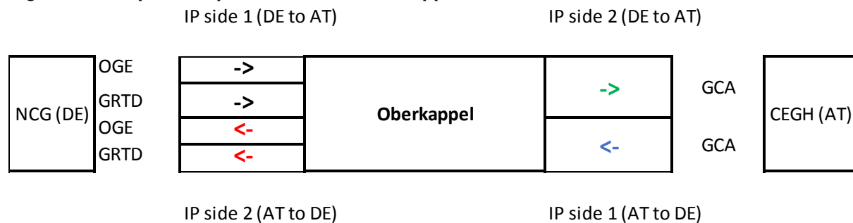
Figure 20: Simplified representation of Oberkappel IP
