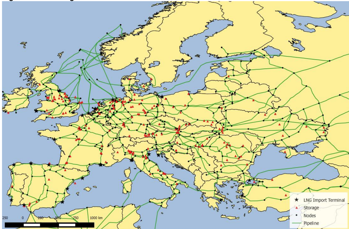
Figure 18: Natural gas infrastructure in TIGER
