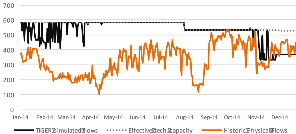
Figure 7: Simulated and historical utilization flows from NCG to Switzerland in 2014 (GWh)
