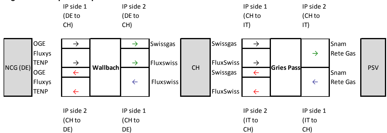
Figure 19: Simplified representation of Wallbach IP and Gries Pass IPs
