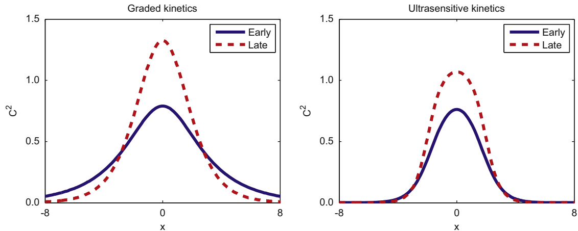
Fig. 7. Comparison of the gradient at the end of the second stage, under graded and ultrasensitive signalling kinetics. The four gradients shown in Fig. 6 are used here as four input gradients to the second stage. With D_1 and \lambda_1 as in Fig. 6, the parameters for the second stage here are D_2^E = 0.9D_1^E , D_2^L = 0.75D_2^E , \lambda_2^E = 0.25\lambda_1^E , \lambda_2^L = 0.9\lambda_2^E . The distinction between graded and ultrasensitive kinetics at this second stage is not as pronounced as at the end of the first stage (compare with Fig. 6).
