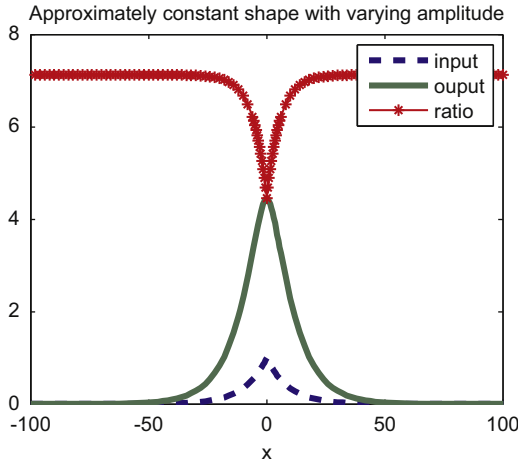
Fig. 8. Quadrature on (6) reveals an example of an input gradient, g = e^{-v|x|} , that results in an output gradient, v , which maintains an approximately constant shape with increasing amplitude. The ratio of output to input, v/g , is also plotted. Parameters are as follows: \lambda = 3.5 , D=2 , \rho = \lambda^2/D + 1 = 7.125 , v = \sqrt{1/\lambda^2 - 1/(\rho D)} \approx 0.1 .
