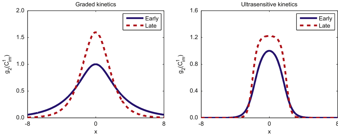
Fig. 6. Comparison of the gradient at the end of the first stage, under graded and ultrasensitive signalling kinetics. Input g_1 is a Gaussian with mean zero and variance \sigma^2 . For these parameters, with ultrasensitive kinetics, the peak broadens at a late stage, which is not consistent with the experimental data, (ii). Parameters for the early stage are the same as Fig. 4. Late stage: D_1^L = D_1^E/3 , \alpha_1^L = 4\alpha_1^E/3 .
