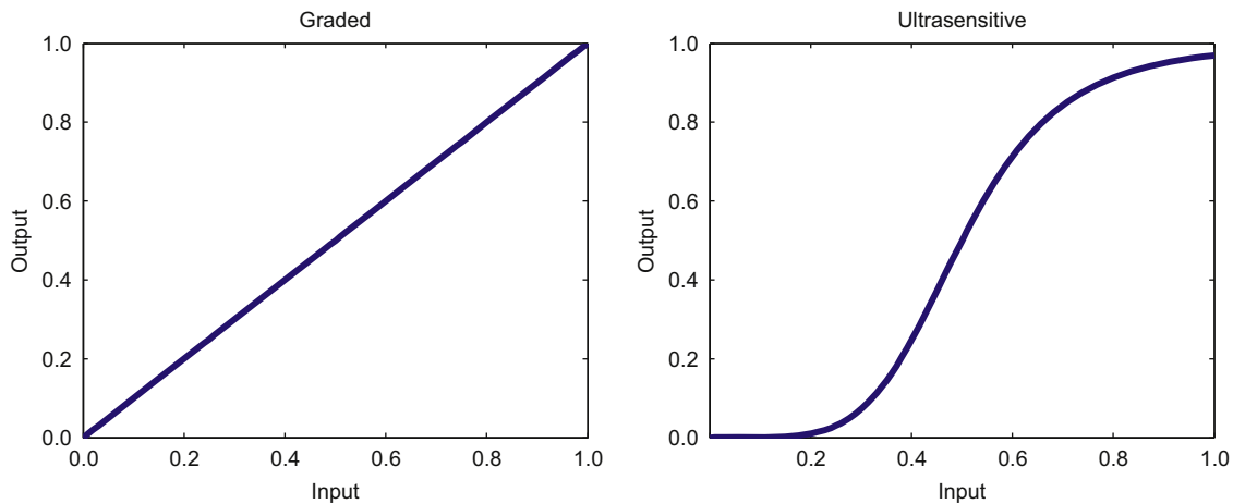
Fig. 3. Example of the relationship of output to input in a graded ( f(x) = cx ) and ultrasensitive ( f(x) = c/(1 + (x_{50}/x)^n) ) function. Parameters: c = 1 , x_{50} = 0.5 and n = 5 .
