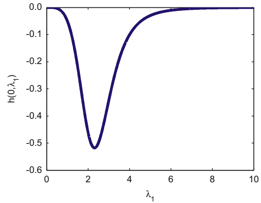
Fig. B1. A unique minimum at 2.3 \approx \lambda_1^* < \sqrt[n]{\hat{C}_{01}} \approx 2.5 . Parameters are as follows: n=5 , \hat{C}_{01} = 100 .
