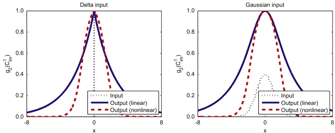
Fig. 4. Comparison of the inputs to the second stage, under graded (linear) and ultrasensitive (nonlinear) signalling kinetics. Input g_1 is a Delta distribution on x=0 (left), or a Gaussian distribution with mean zero and variance \sigma^2 (right). For the Delta distribution input the effective length scale is reduced by a factor of n=5 by the ultrasensitive MAPK signalling kinetics. Parameters are as follows: D_1=0.5 , \alpha_1=1.5 , \beta_1=2 , k_{im}^{(1)}=0.1 , k_m^{(1)}=0.01 , \lambda_1=2.0 , K_1=2.0 , D_1=1.0 , \sigma^2=1.0 . For the Hill function parameters in (7) we set C_0=1.0 and n=5 and in each case we choose the scale factors g_l and g_n so the peak is unity: g_l=0.565 and g_n=1.0576 (left), and g_l=0.7586 and g_n=1.2512 (right).
