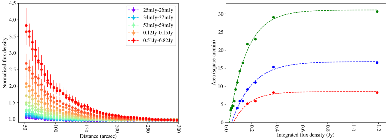
Fig. 11. Left panel: profiles of the average standard deviation as a function of distance from compact LoTSS-DR1 sources in various integrated flux density bins. The integrated flux density bins were chosen to contain equal numbers of sources (110) and they vary from 25.0 mJy to 26.2 mJy (blue) to 510 mJy to 6820 mJy (red). The errors are 95% confidence intervals on the median values derived from the bootstrap method. Right panel: an estimate of the area in which the noise is 15% (green), 50% (blue), and 100% (red) higher than the thermal noise due to dynamic-range limitations around a bright source; the points show the measured values and the dotted lines show the best-fitting curves.
