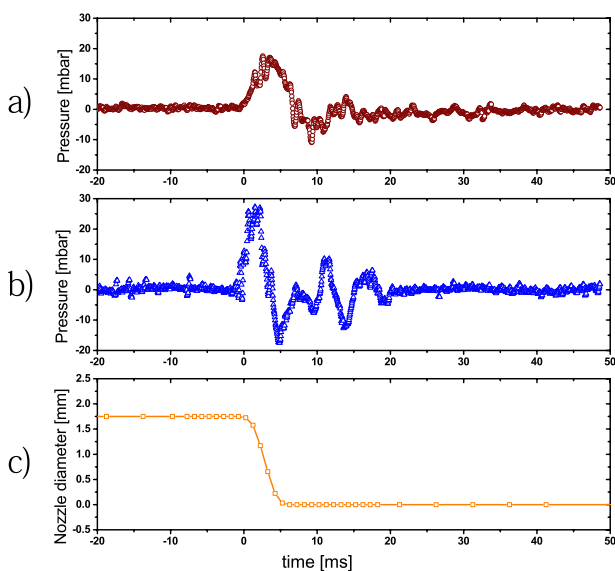
FIG. 3. Pressure waveforms used during these experiments. The waveform in (a) jets droplets with a short filament attached at 1.10 m s -1 for non-dynamical nozzles of 1.75 mm diameter. Waveform (b) jets droplets with a long ligament at 1.80 m s -1 for non-dynamical nozzles of 1.75 mm diameter. (c) shows the nozzle diameter as it varies in time after the closing action begins 1.25 ms after the arrival of the pressure pulse.
