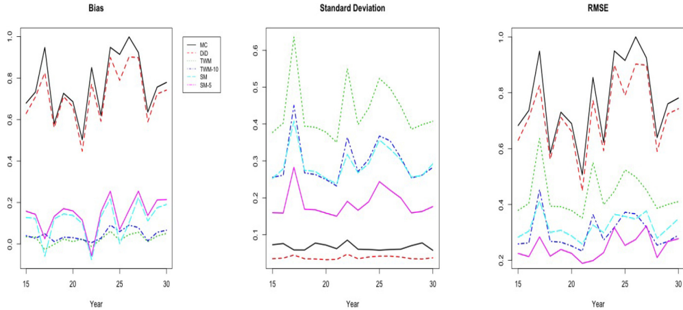
Figure 4. Results for t \mapsto \mu_t(0 | \{1\}) .
