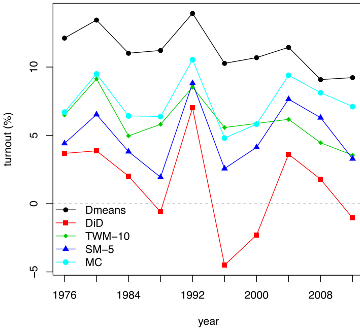
Figure 2. Average treatment effect on treated.
