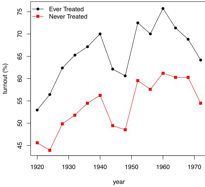
Figure 1. Pre-trends in turnout rate.
