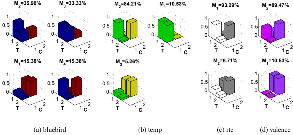
Figure 7: Mean confusion matrices of the user’s clusters identified by hcBCC. M_i denotes the percentage of users allocated to cluster i , T is the ground truth label, and C is the user label.
