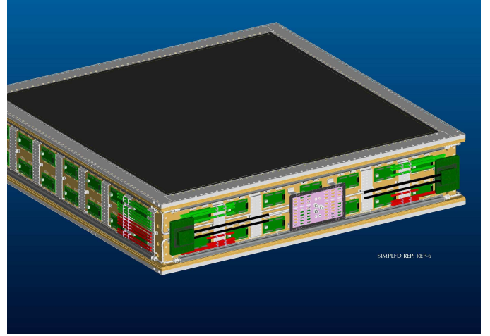
Figure 23: External view of one ECal module. The scintillator bars run horizontally inside the module as shown. The readout electronics, signal and power cables, and cooling pipes can be seen mounted on the aluminum plates on the sides of the module. The gray surface at the top is the carbon fiber sandwich front plate, which in the final module position is facing towards the inner subdetectors (PØD, FGDs and TPCs).
