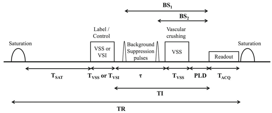
FIGURE 2 Schematic sequence diagram of VSASL (based on Figure 3 in Qin et al. 6 ). Abbreviation: BS, background suppression; TI, inversion time; T_{sat} , saturation time; VSASL, velocity-selective arterial spin labeling; VSI, velocity-selective inversion; VSS, velocity-selective saturation.
