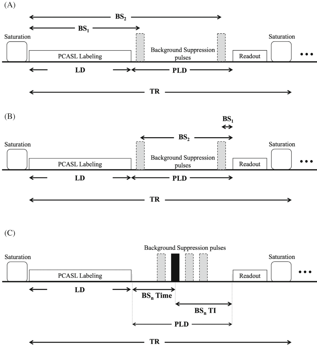
FIGURE 3 Schematic sequence diagram of PCASL. The timing parameter for the BS pulses. In this example, two BS pulses are used. Currently, there are three different definitions of the timings implemented in commercial scanners: (A) time from the center of the first PCASL labeling pulse to the center of the Nth BS pulse, (B) time from the center of the first excitation pulse to the center of the Nth BS pulse, (C) BS_n Time: from the center of the last PCASL labeling pulse to the center of the Nth BS pulse; BS_n TI: from the center of the Nth BS pulse to the center of the first excitation pulse (Figure [c] courtesy: Canon Medical Systems Corporation) Abbreviation: BS, background suppression; LD, labeling duration; PCASL, pseudo-continuous arterial spin labeling; PLD, post-labeling delay; TI, inversion time; TR, repetition time.
