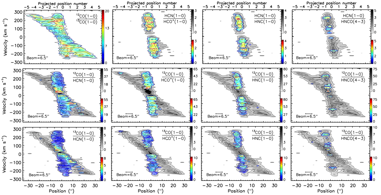
Figure 9. Same as Figures 7 and 8 but for NGC 5866.
