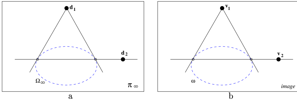
Figure 2. Orthogonality represented by the pole-polar relationship. (a) On \pi_\infty orthogonal directions d_1, d_2 are conjugate wrt \Omega_\infty . (b) On the image plane orthogonal rays v_1, v_2 are conjugate wrt \omega .
