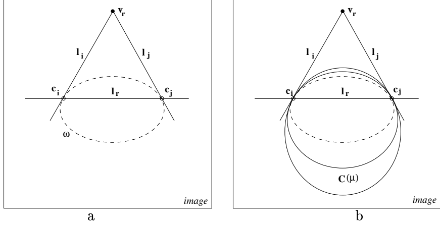
Figure 3. (a) The image fixed points and lines under a rotation, and their relation to \omega . The point \mathbf{v}_r is the vanishing point of the rotation axis direction, and \mathbf{c}_i and \mathbf{c}_j are the imaged circular points for planes orthogonal to the rotation axis. The line \mathbf{l}_r is the vanishing line for planes orthogonal to the rotation axis. The image of the absolute conic contains the imaged circular points. The point \mathbf{v}_r and line \mathbf{l}_r have a pole-polar relationship wrt \omega ; with \omega tangent to the lines \mathbf{l}_i, \mathbf{l}_j at the imaged circular points. (b) These relations do not uniquely define the conic \omega . There is a pencil of conics \mathcal{C}(\mu) consistent with the constraints.
