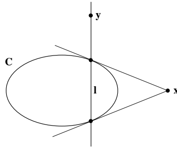
Figure 1. The pole-polar relationship. The line l = Cx is the polar of the point x wrt the conic C , and the point x = C^{-1}l is the pole of l wrt C . The polar of x intersects the conic at the points of tangency of lines from x . If y is on l then y^T l = y^T Cx = 0 . Points x and y which satisfy y^T Cx = 0 are conjugate .
