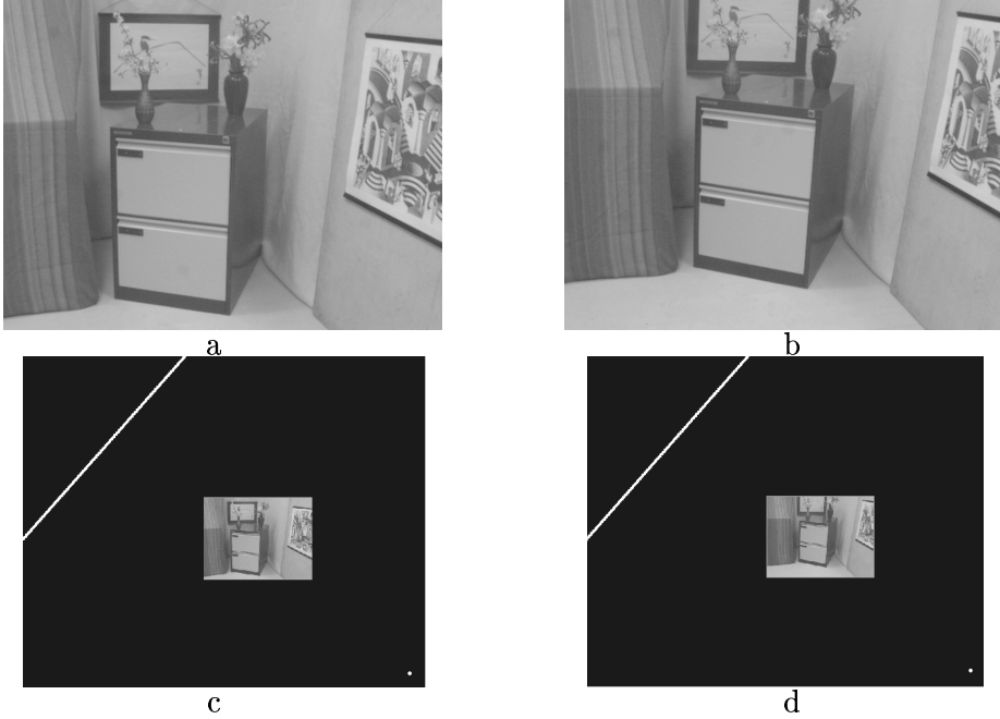
Figure 5. The motion between (a) and (b) is a rotation about the camera centre, with the rotation axis not aligned with with the image axes. (c) and (d) show the fixed point and line computed from the eigenvectors of \mathbf{H}_\infty .
