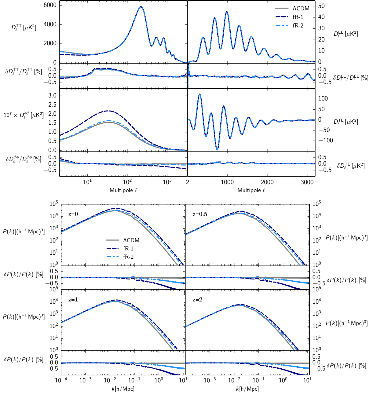
Figure 6. f(R) . Top figure: The TT , EE , lensing and TE angular power spectra of the CMB for two different f(R) models and a reference \Lambda CDM along with the relative difference between EFTCAMB and CLASS_EOS_fR. Bottom figure: The same as in the top figure but for the matter power spectrum at different redshifts. The exact values for the cosmological parameters used here can be found in Appendix B 3.
