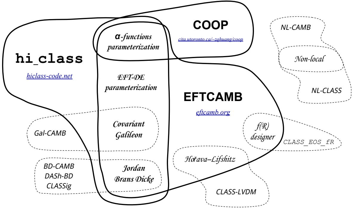
Figure 1. Overlap between codes and theories used in the comparison. Each code is represented by a silhouette that covers the models for which it has been compared. General-purpose and publicly available codes are represented by thick solid regions, while model-specific or private codes are enclosed by dashed lines. Note that we only show the models used in this paper, not the full theory space available to each code.
