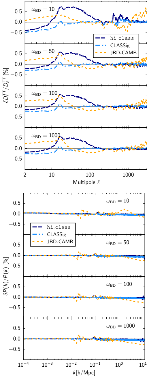
Figure 3. JBD. Top figure: The relative difference of the TT angular power spectra of the CMB for the same models showed in Fig. 2. Every panel corresponds to a model and the comparison of each code in the legend – CLASSig , JBD-CAMB and hi_class for reference – has been done w.r.t. EFTCAMB . Bottom figure: The same as in the top figure but for the matter power spectrum.
