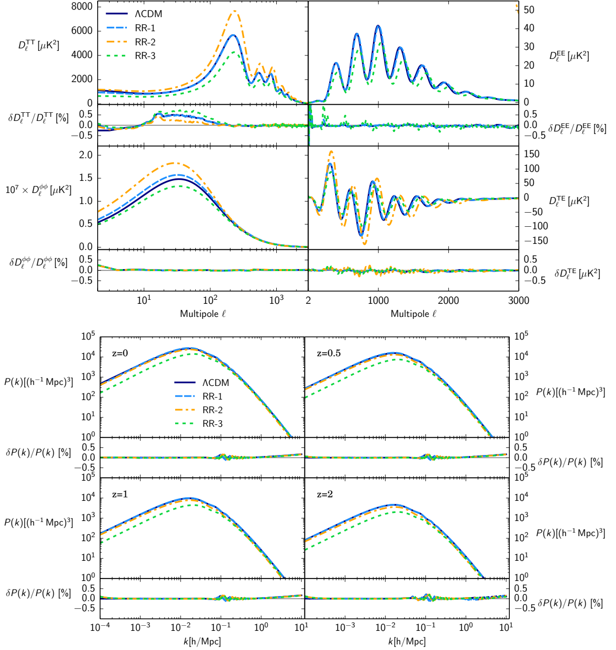
Figure 7. Non-local Gravity. Top figure: The TT , EE , lensing and TE angular power spectra of the CMB for three different Non Local Gravity models along with the relative difference between RR-CAMB and RR-CLASS. Bottom figure: The same as in the top figure but for the matter power spectrum at different redshifts. The exact values for the cosmological parameters used here can be found in Appendix B 4.
