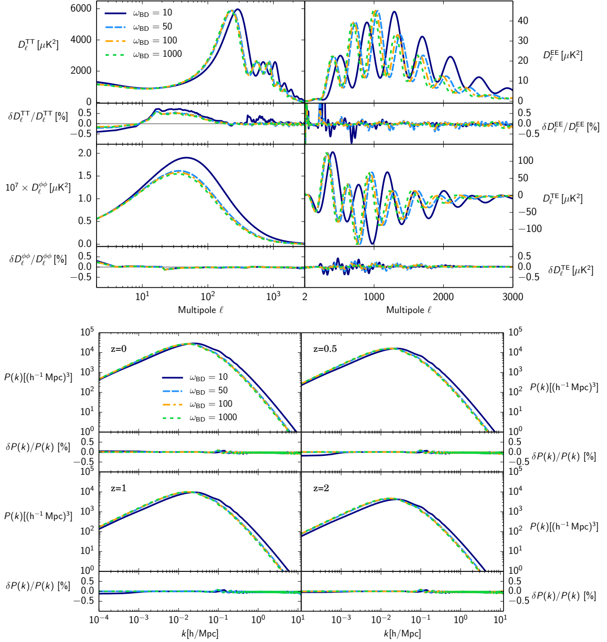
Figure 2. JBD. Top figure: The TT , EE , lensing and TE angular power spectra of the CMB – with D_\ell^{XY} \equiv \ell(\ell+1)/2\pi C_\ell^{XY} – for a range of values of \omega_{BD} along with the relative difference between EFTCAMB and hi_class. Bottom figure: The same as in the top figure but for the matter power spectrum at different redshifts. The exact values for the cosmological parameters used here can be found in Appendix B 1.
