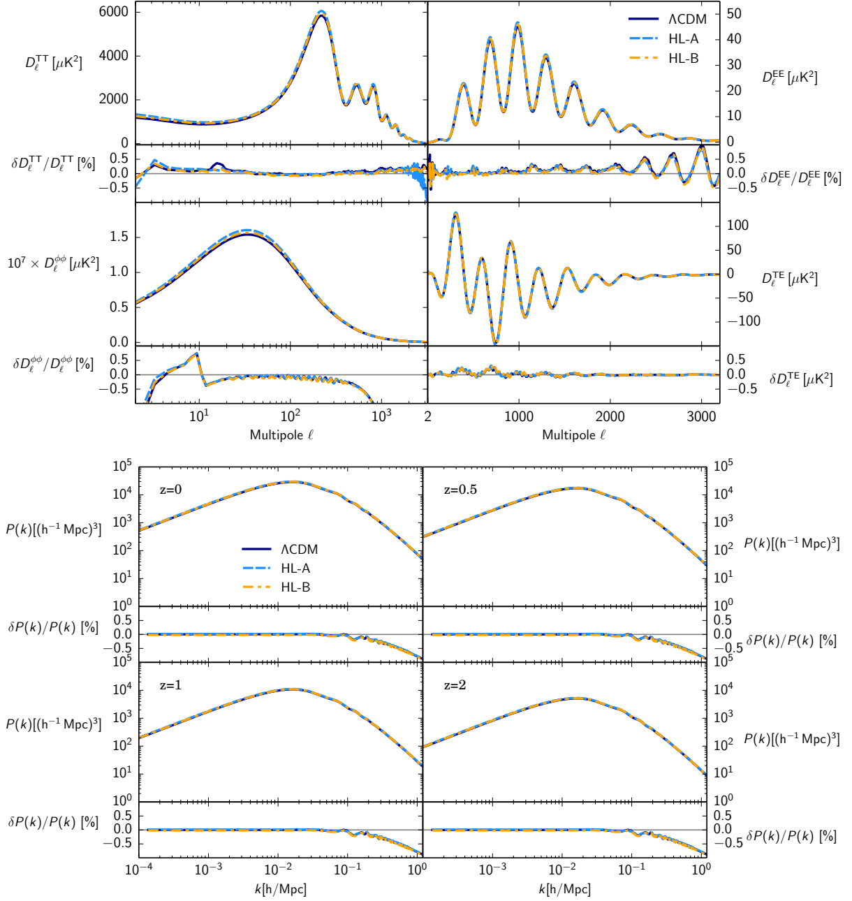
Figure 8. Hořava-Lifshitz Gravity. Top figure: The TT , EE , lensing and TE angular power spectra of the CMB for two different Hořava-Lifshitz models along with the relative difference between EFTCAMB and CLASS-LVDM. Bottom figure: The same as in the top figure but for the matter power spectrum at different redshifts. The exact values for the cosmological parameters used here can be found in Appendix B 5.
